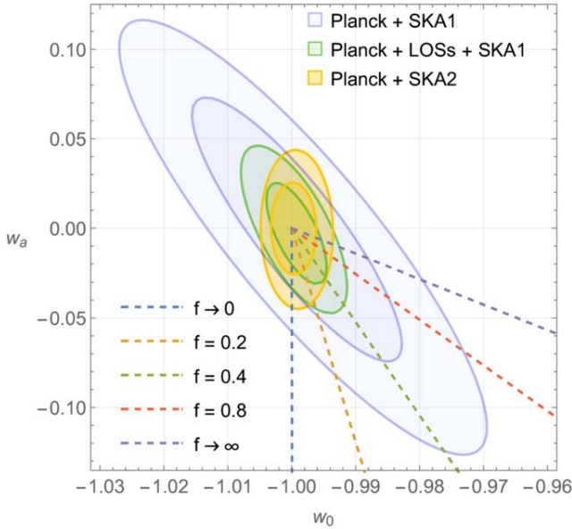
Figure 7. Comparison between the expected 67% and 95% CL constraints on w_0 – w_a from various future experiments (blue, green, and yellow ellipses) and the w_0 – w_a relation for the thawing model described by the potential given in Equation (16) for different values of the parameter f .
