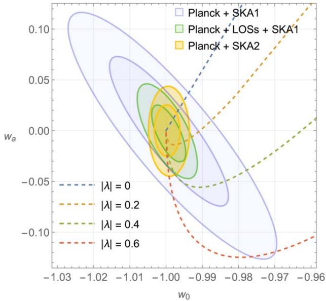
Figure 3. Relation between w_0 , w_a and |\lambda_0| = |V'(0)|/V(0) . The ellipses represent the expected 67% and 95% CL constraints on w – w_a from various future experiments, while the dashed lines are the isolines \lambda = \text{constant} as calculated with Equation (8) evaluated at N = 0 .
