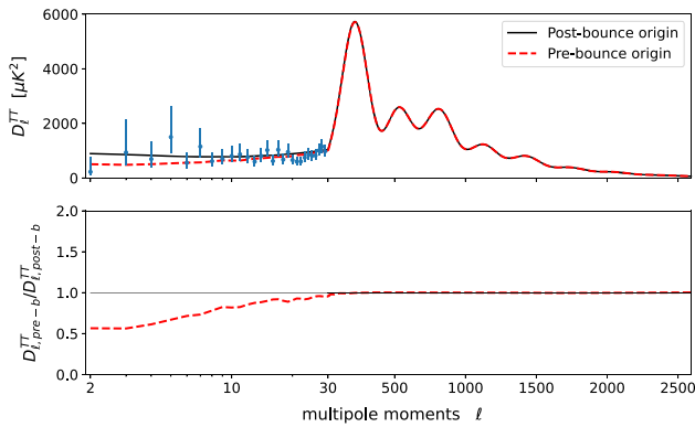
Fig. 10 Temperature angular power spectra D_{\ell}^{TT} for a pre-bounce and for a post-bounce origin of structures, with background IC \{-0.467, +1\} , and a quadratic potential. Top: D_{L,\text{post-b}}^{TT} in black, D_{\ell,\text{pre-b}}^{TT} in dashed red, Planck data in blue. Bottom: Ratio of the spectra in dashed red
