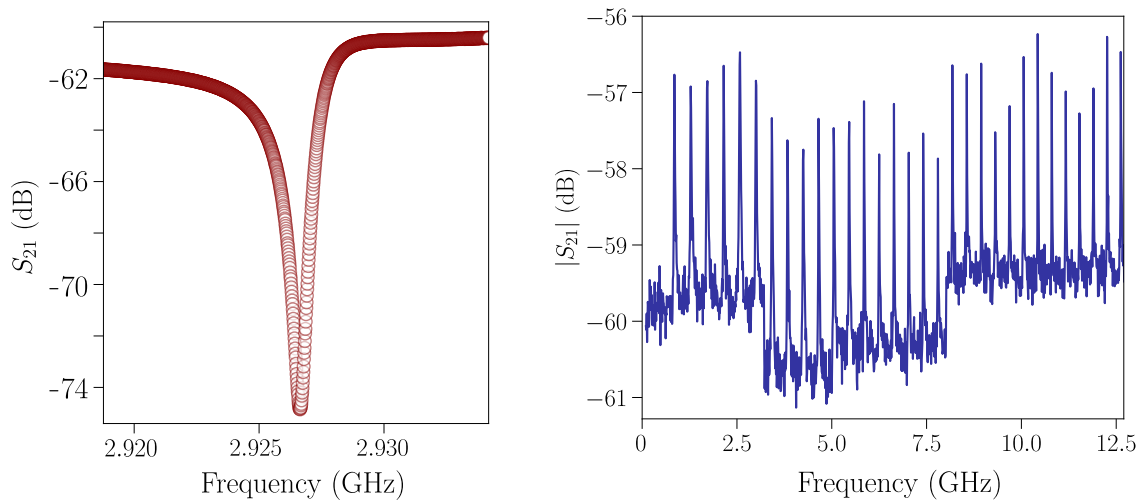
Fig. 5.2. a) Typical microwave transmission near a resonant mode of an indium oxide stripline, characterized by a drop in amplitude. b) Excerpt of a typical two-tones measurement displaying a series of transmission peaks, each of which signals the existence of a resonant mode.
