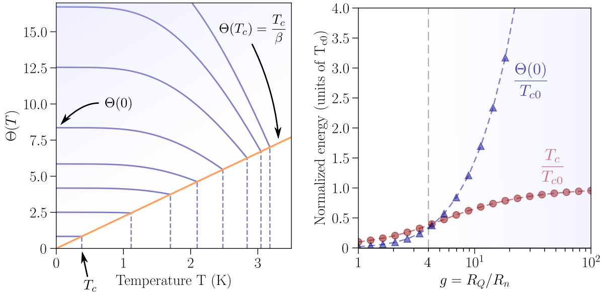
Fig. 5.6. Suppression of critical temperature with normal-state conductance via the BKT mechanism. Left: Result of the numerical solving of Eq. (5.6). Orange line is the BKT relation \Theta(T_c) = T_c/\beta . The superfluid stiffness decreases with temperature as the number of quasiparticles increases following the Mattis-Bardeen formula (this is the main difference with Fig. 1.2). At T = T_c where the BKT jump of \Theta occurs, superconductivity is suppressed abruptly. As disorder is increased ( g decreased) the value of \Theta(T_c) at the BKT transition gets closer to the zero- T value \Theta(0) . Eventually, for sufficiently strong disorder T_c \sim \beta\Theta(0) . Right: Resulting T_c and \Theta(0) (in units of the mean-field critical temperature T_{c0} ) versus normal-state conductance. Upon decrease of g both energy scales are reduced, and below g = 4 the critical temperature is ruled by phase fluctuations as can be seen from the proportionality T_c \propto \Theta(0) .
