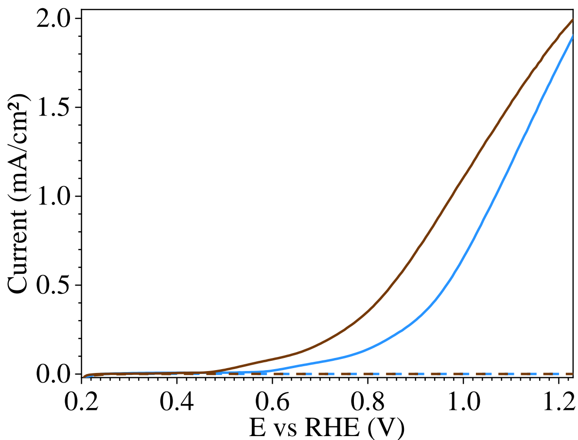
Figure A.1: Photoelectrochemical measurements in 1M potassium phosphate buffer (pH 6) under front simulated illumination at 100 mW cm -2 . Linear voltage sweeps of Mo:BiVO 4 /Co-Pi (5 min) with 1 h calcination at 450 °C for Mo:BiVO 4 in blue curve and 3 h calcination at 450 °C for Mo:BiVO 4 in brown curve. The dots are measured under dark condition.
