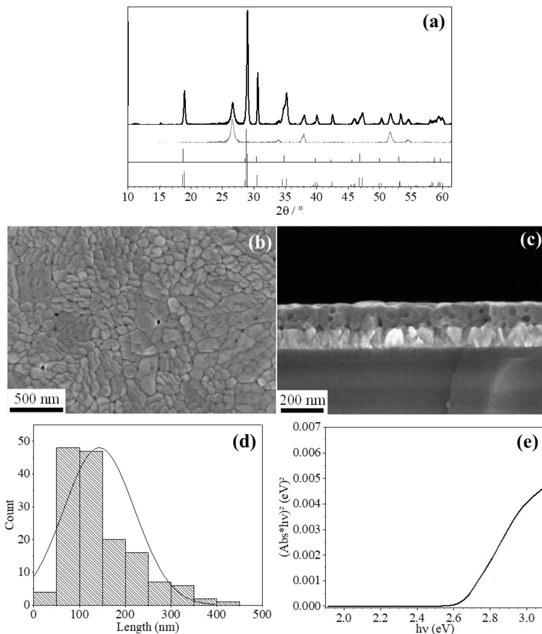
Figure 1: pristine \text{BiVO}_4 characterisation: a) XRD pattern of pristine \text{BiVO}_4 (black curve), grey curve annealed FTO substrate (grey curve), PDF-04-010-5710 \text{BiVO}_4 tetragonal scheelite (blue straight-line ) and PDF-04-010-5713 \text{BiVO}_4 monoclinic scheelite (black straight-line); b)FEG-SEM surface imaging; c) FEG-SEM cross-section imaging e) Bang-gap determination by ellipsometry
