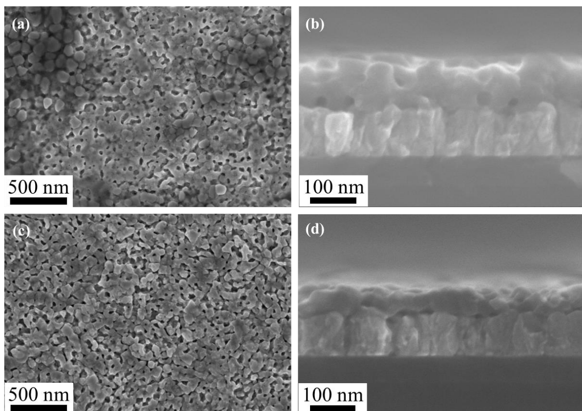
Figure S14: FEG-SEM post-mortem after PEC analysis under back-illumination of a) \text{BiVO}_4 surface, b) \text{BiVO}_4 cross-section c) \text{Mo:BiVO}_4 surface, d) \text{Mo:BiVO}_4 cross-section.
