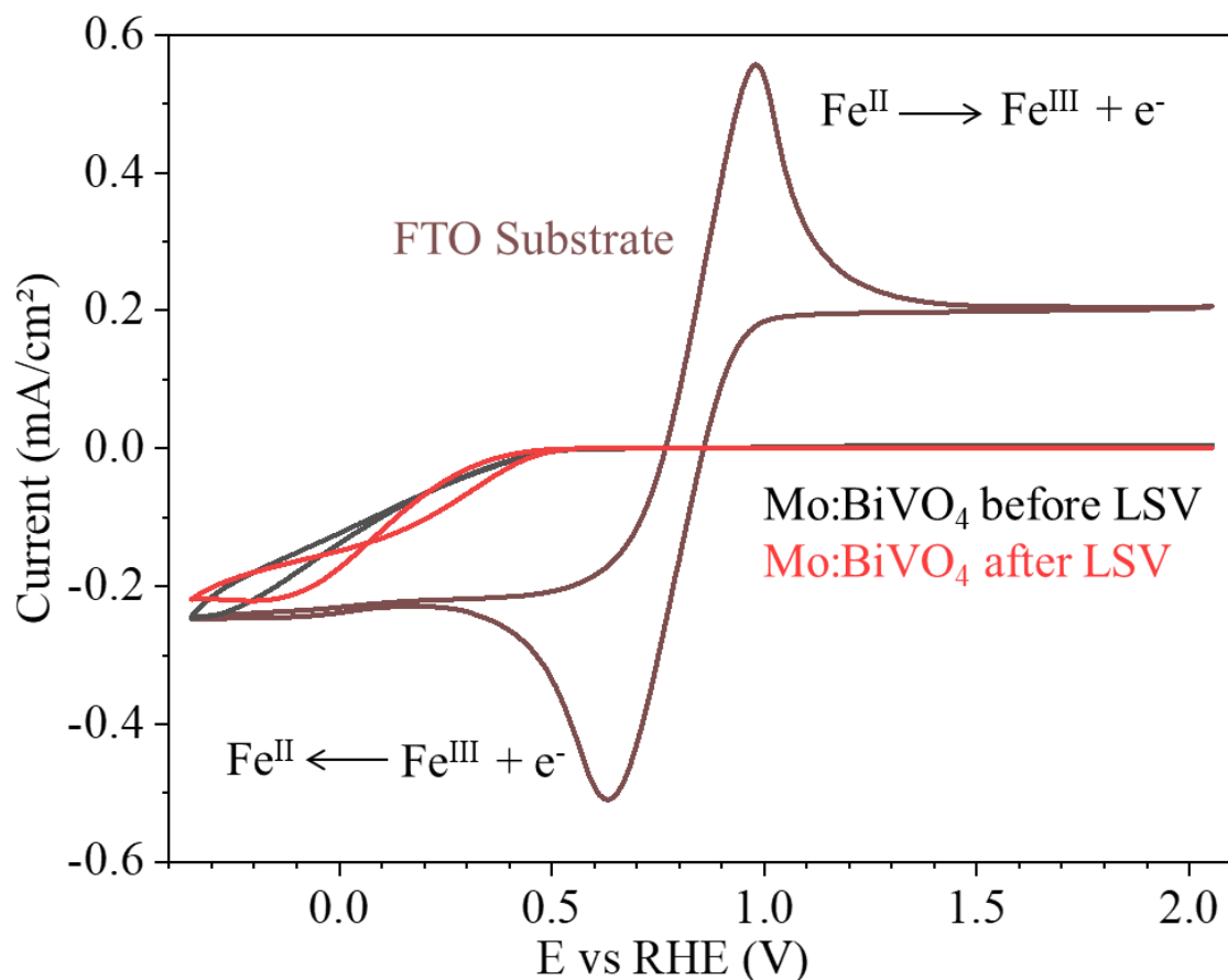
Figure S17: Oxidation and reduction \text{Fe}^{3+}/\text{Fe}^{2+} study by cyclic voltammetry on naked FTO, \text{Mo:BiVO}_4 before any photoexcitation (in black) and after several linear sweep voltammetry measurements in dark and light modes (in red)
