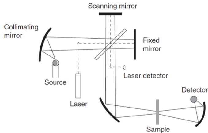
Figure 2.1: The optical arrangement of an FT-IR spectrometer. Figure extracted from [4].
