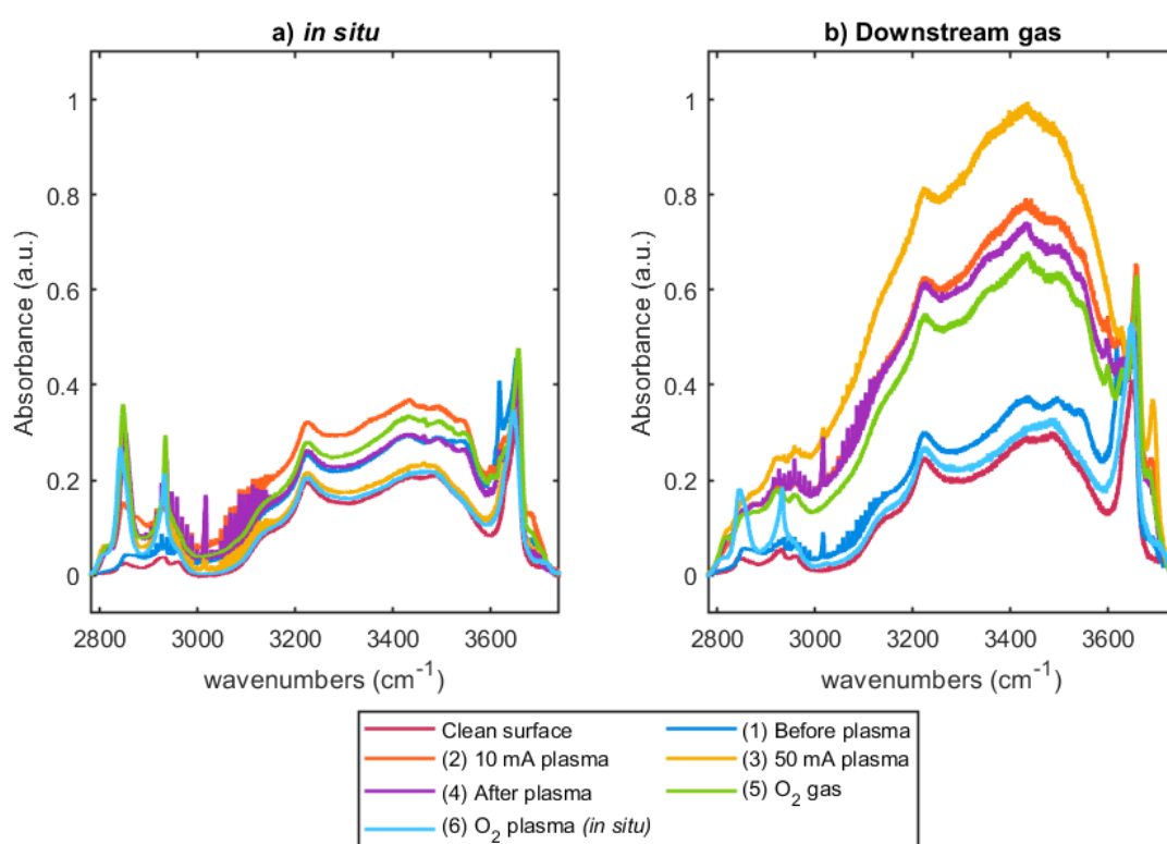
Figure 5.6: FTIR transmission spectra of 70%CO 2 -30%CH 4 plasma at 1 torr in the region 2800 - 3700 cm -1 typical of OH groups for in situ experiments (a) and downstream gas experiments (b). Each spectrum is the final spectrum taken after each step from the experimental sequence.
