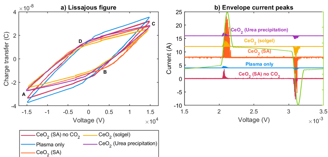
Figure 8.22: a) Lissajous figure and b) envelope of the current in the positive V from experiments for plasma only and with CeO 2 (SA), CeO 2 (SA) no CO 2 , CeO 2 (solgel) and CeO 2 (Urea precipitation) in 70%CO 2 -30%CH 4 plasma PB-DBD, 15 kV amplitude (30 kV peak-to-peak), 750 torr. The envelope corresponds to the accumulation of 1000 periods. The envelope is offset for clarity. One voltage cycle (green) is presented for further discussion.
