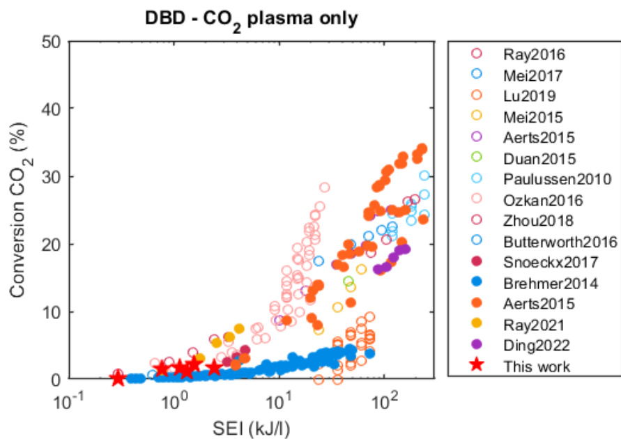
Figure 8.24: Conversions of CO 2 as a function of SEI for DBD plasmas in pure CO 2 extracted from literature using the PIONEER database tool ( www.db.co2pioneer.eu , date of extraction: 21/02/2023). Data from this work are shown as red stars.
