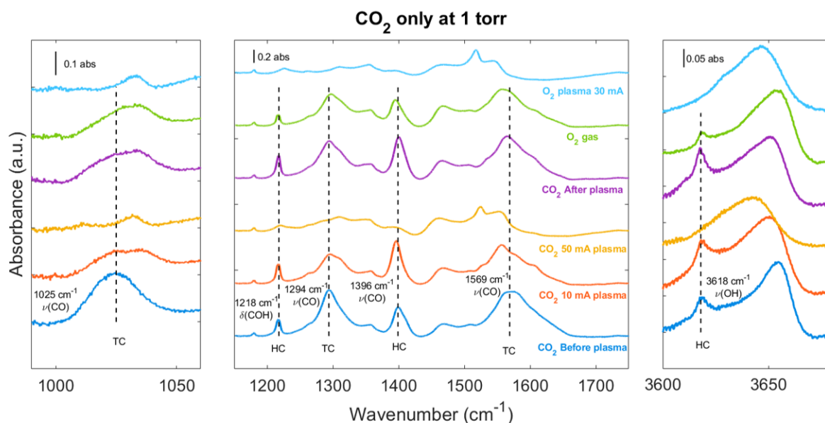
Figure 3.14: In situ FTIR transmission spectra of CO 2 adsorbed as carbonates species during CO 2 only experiments in ceria surface at 1 Torr in the cross DC glow discharge plasma reactor through the experimental sequence. TC: Tridentate carbonates, HC: Hydrogen carbonates. The spectra displayed corresponds to the final spectrum taken at the end of each step from the experimental sequence. Spectra are offset for clarity.
