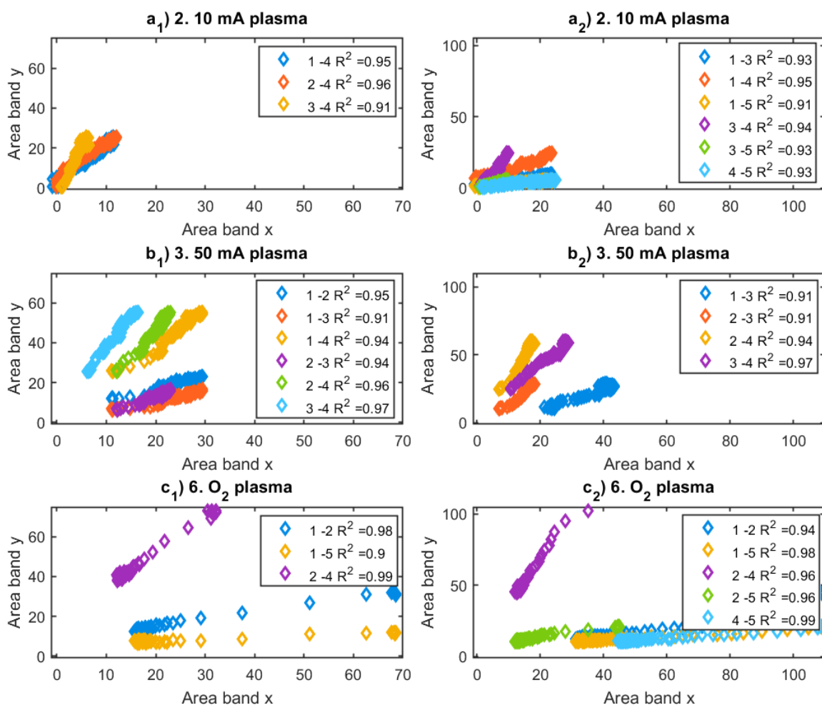
Figure 3.19: Correlation of bands x vs y during in situ transmission experiments for 70%CO 2 -30%CH 4 at 1 Torr (a 1 , b 1 and c 1 ) and 5 Torr (a 2 , b 2 and c 2 ). Numbers are assigned to a specific band: 1 = 1358 cm -1 , 2 = 1370 cm -1 , 3 = 2722 cm -1 , 4 = 2845 cm -1 and 5 = 2933 cm -1 . Coefficient of determination R 2 is shown for every band correlated with more than 0.9.
