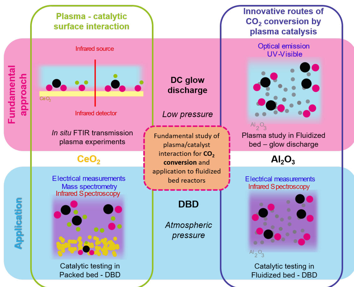
Figure 1.4: Schematic correlating the fundamental approach and application study for plasma-catalytic surface interaction with fluidized bed plasma reactors as innovative route for CO 2 conversion by plasma catalysis described in this thesis work.
