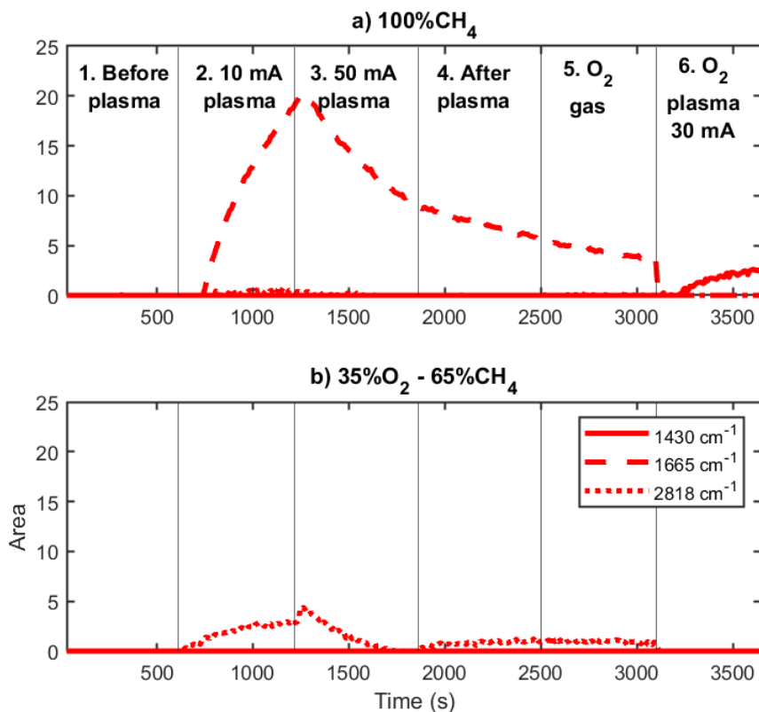
Figure 6.13: Time evolution of the area corresponding to 1430\text{ cm}^{-1} (solid line), 1665\text{ cm}^{-1} (dashed line) and 2818\text{ cm}^{-1} (dotted line) bands for a) 100\%\text{CH}_4 plasma and b) 35\%\text{O}_2\text{-}65\%\text{CH}_4 plasma at 1 Torr during in situ FTIR transmission experiments.
