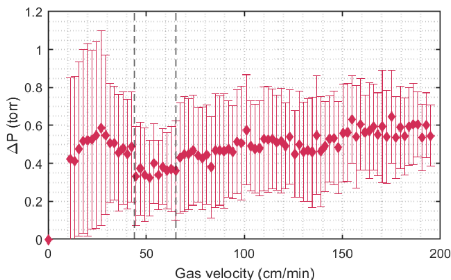
Figure 9.2: Pressure drop as a function of gas velocity caused by the presence of 0.3 g \text{Al}_2\text{O}_3 bed. The error bars represent \pm standard deviation from 3 separated measurements.
