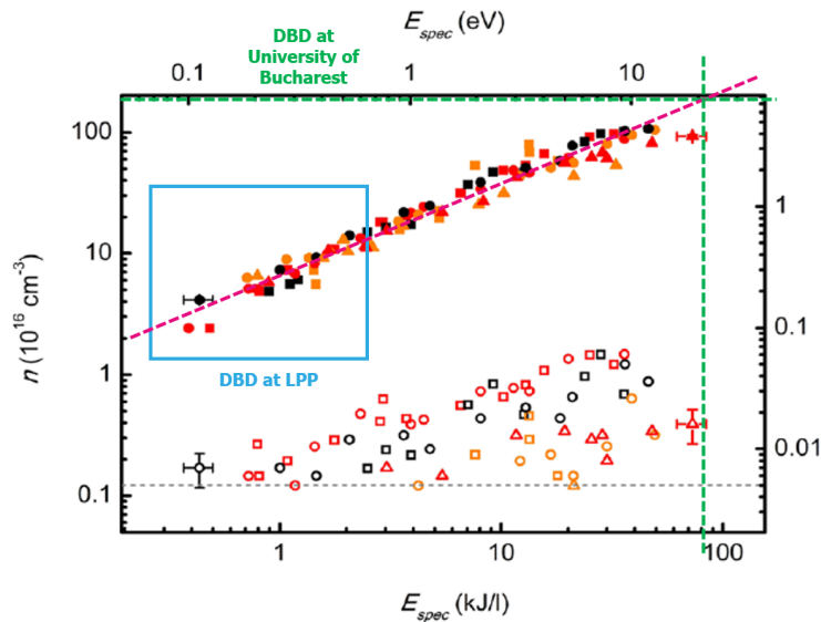
Figure 8.15: Figure extracted from [19] showing the densities of CO (full marker) as a function of specific energy input. Pink dashed line represents the trend followed by the measurements reported in the paper. Green dashed line shows the CO density and corresponding specific energy input from the results obtained by the DBD at University of Bucharest for pure \text{CO}_2 plasma. The light blue box points the region of CO density and SEI expected for the results shown in this chapter.
