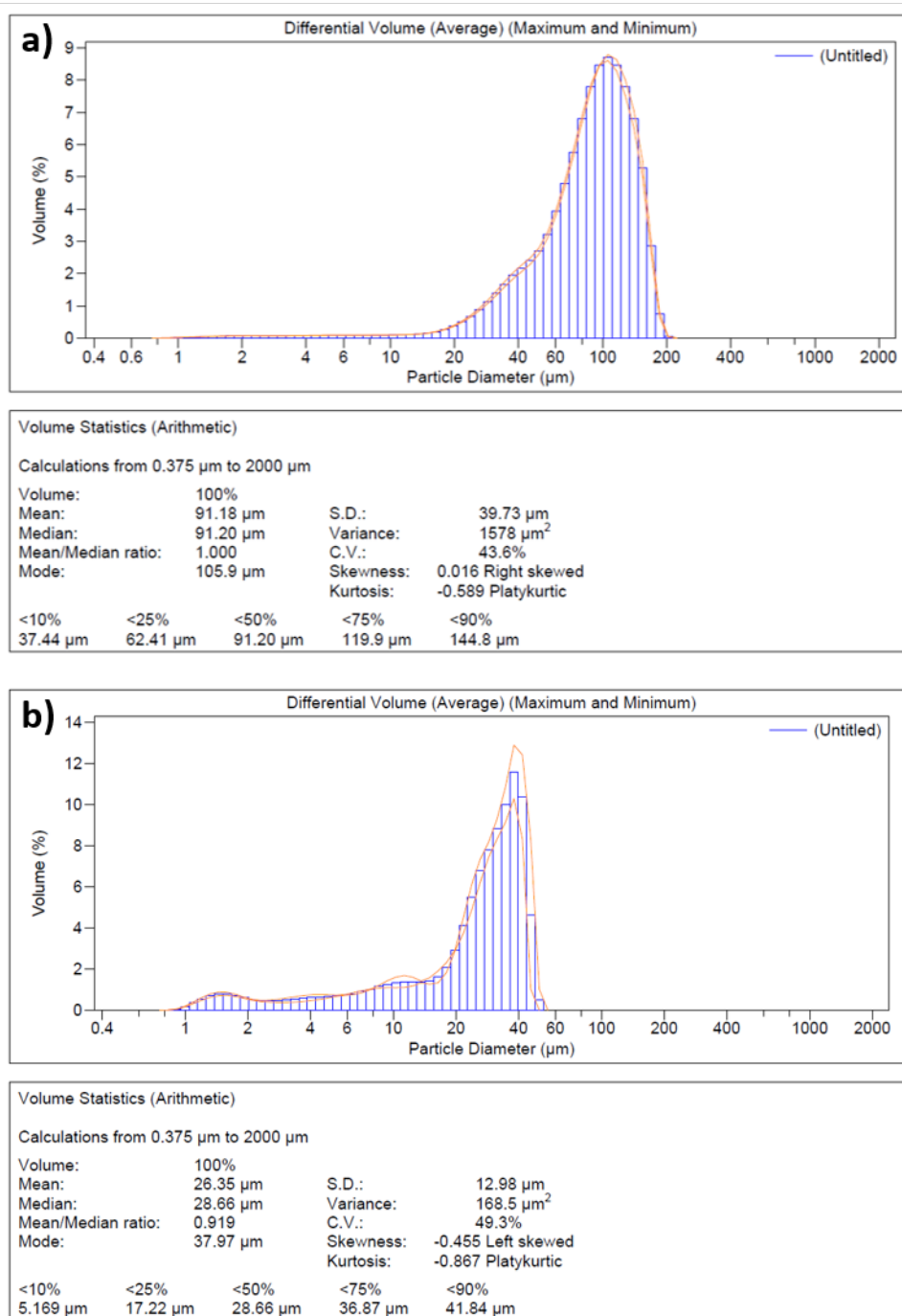
Figure 7.27: Particle size analysis of Al 2 O 3 a) before and b) after plasma treatment in FB-GD. Analysis carried out by Instituto de Carboquímica in Zaragoza, Spain.
