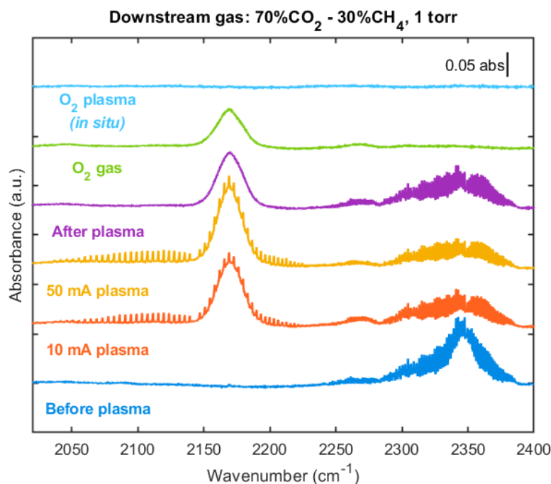
Figure 5.11: Region 2050 - 2400 \text{cm}^{-1} FTIR spectra showing CO and CO 2 gas phase bands from downstream gas of 70%CO 2 - 30%CH 4 plasma experiments at 1 Torr. Spectra are offset for clarity.
