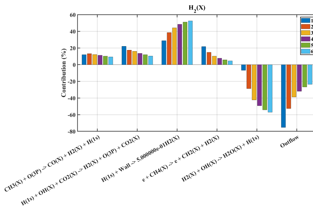
Figure D.1: Evolution of contribution of the main creation and destruction processes for H 2 for 95%CO 2 -5%CH 4 plasma at 30 mA, 20 sccm from 1 to 6 Torr.
