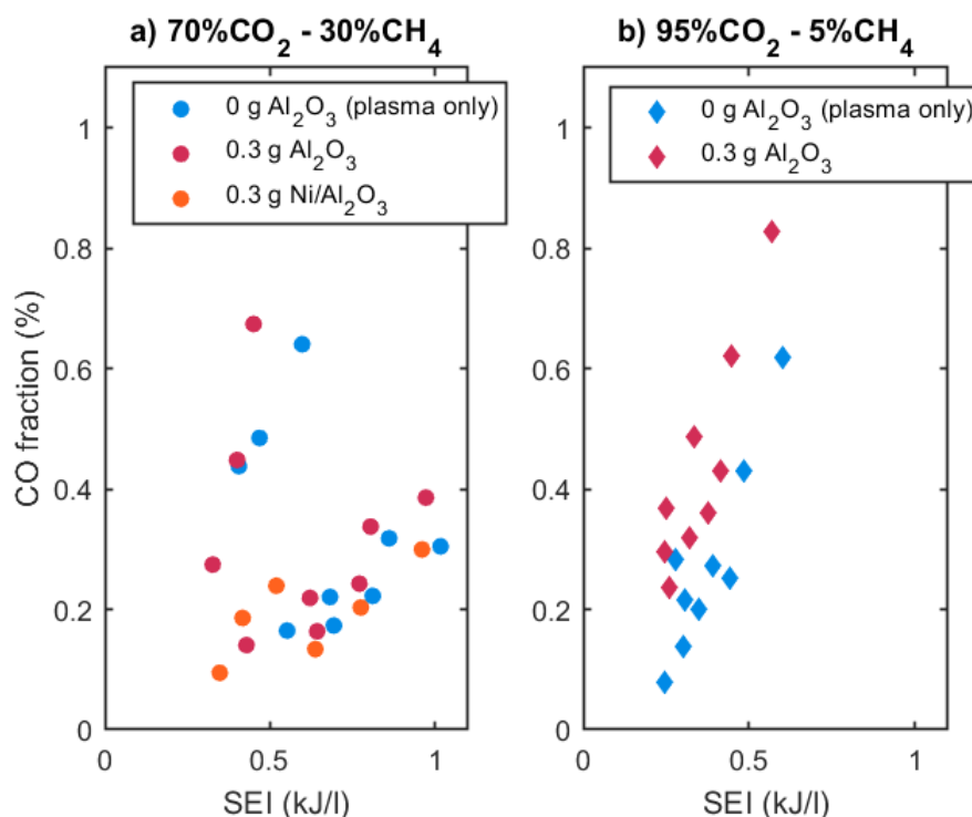
Figure 9.7: CO fraction as a function of SEI for a) 70%CO 2 -30%CH 4 and b) 95%CO 2 -5%CH 4 initial gas mixtures.
