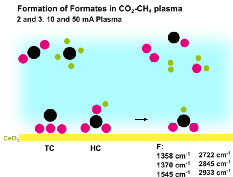
Figure 3.20: Scheme of formate formation in CeO 2 surface during CO 2 -CH 4 plasma steps (2 and 3) based on the bands observed corresponding formates.
