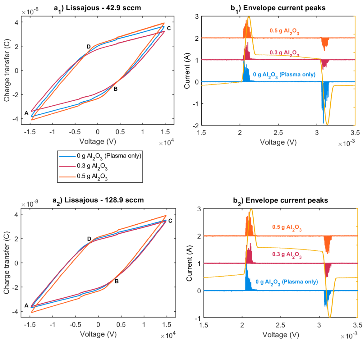
Figure 9.5: Lissajous plots of CO 2 plasma at a 1 ) 42.9 sccm and a 2 ) 128.9 with the corresponding envelope current peaks in b 1 ) and b 2 ), respectively for 0 g Al 2 O 3 (plasma only), 0.3 and 0.5 g of Al 2 O 3 . Voltage: 15 kV amplitude (30 kV peak-to-peak); Pressure: 750 torr.
