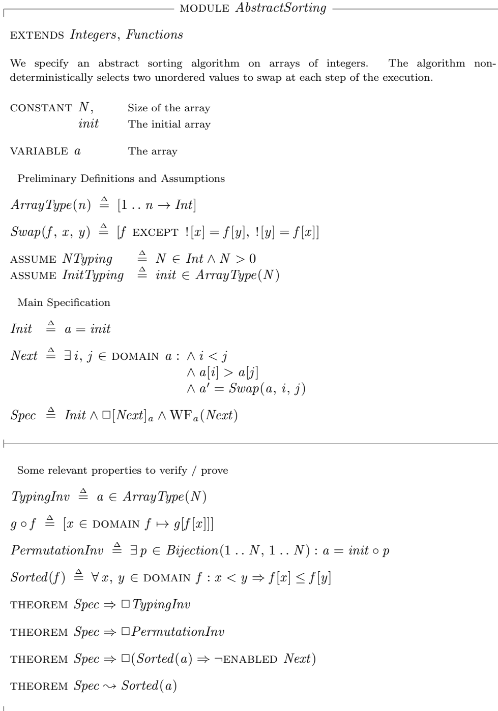
Figure 2.3: Abstract Specification of a Sorting Algorithm
