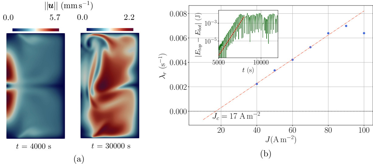
Figure 3.4 – Determination of the threshold of unsteadiness. (a) Velocity distribution for J = 50 A m -2 at t = 4000 s and at t = 30000 s (b) On the inset graph is plotted the difference |E_{top} - E_{bot}| for J = 50 A m -2 . The growth rate \lambda_r of this difference, which corresponds to the slope of the increasing part, is plotted in blue for different J . A linear fit of these values (orange dashed line) leads to the threshold J_c = 17 A m -2 .
