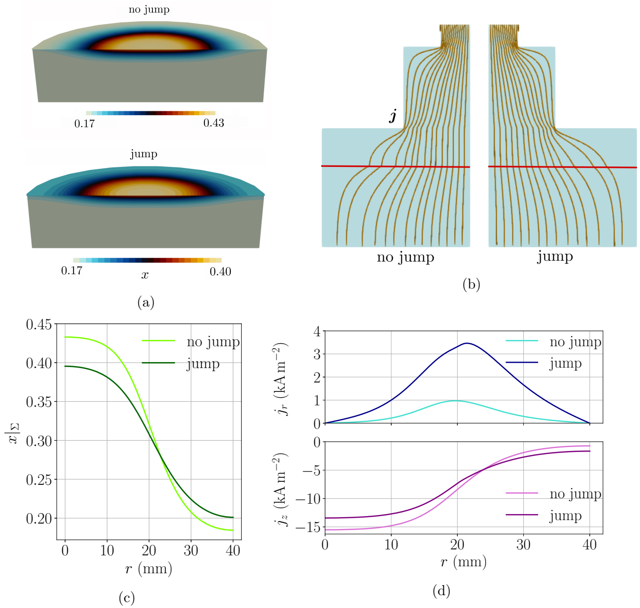
Figure 5.13 – I= 10 A. Molar fraction in the alloy and current density in pure diffusive case, at t = 500 s, with or without jump coupling. (a) Snapshots of the molar fraction of lithium in the alloy x . (b) Streamlines of the current density in the cell. (c) Molar fraction x|_{\Sigma} at the alloy-electrolyte interface as a function of radius r .(d) Current density j_r (top) and j_z (bottom) at the alloy-electrolyte interface as a function of radius r .
