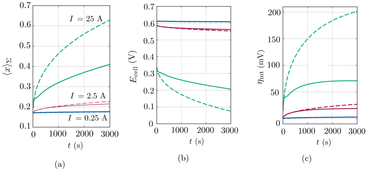
Figure 2.3 – Comparison of the pure diffusion case and the numerical results with EVF for three currents, I = 0.25 A (blue), I = 2.5 A (red), I = 25 A (green) as a function of time. (a) Averaged molar fraction at the alloy-electrolyte interface. (b) Potential of the cell. (c) Mass transfer overpotential.
