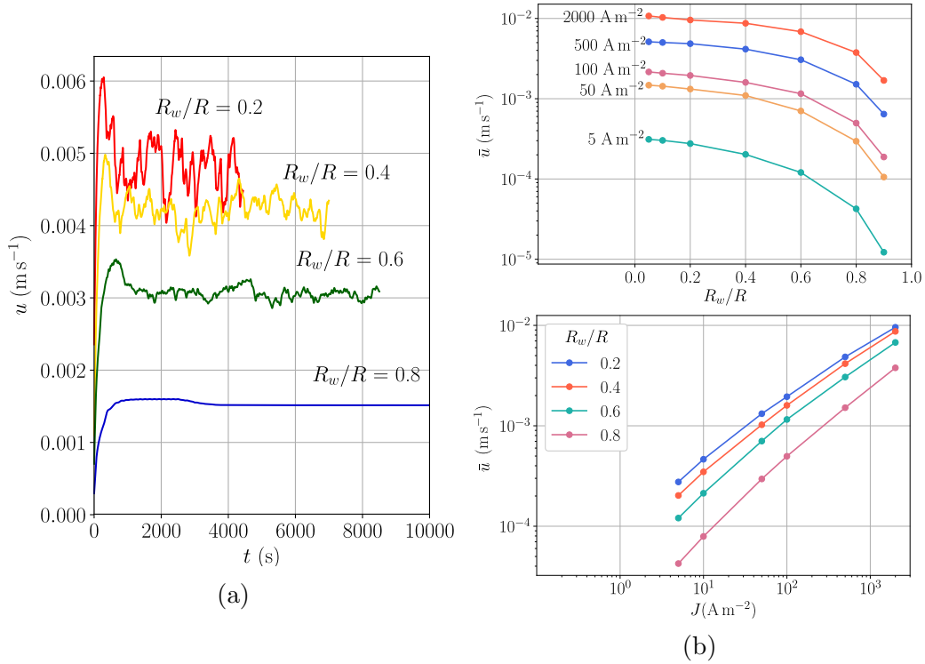
Figure 3.17 – (a) Evolution of the velocity u with time for different R_w/R and J = 500 \text{ A m}^{-2} . (b) Time- and volume-averaged velocity \bar{u} as a function of R_w/R for different J (top), as a function of J for different R_w/R (bottom).
