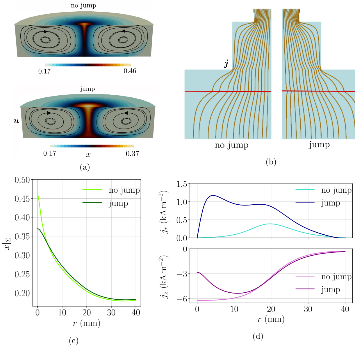
Figure 5.14 – I = 10 A. Molar fraction in the alloy and current density in the case with EVF and no buoyancy, at t = 500 s, with or without jump coupling. (a) Snapshots of the molar fraction of lithium in the alloy x . (b) Streamlines of the current density in the cell. (c) Molar fraction x|_{\Sigma} at the alloy-electrolyte interface as a function of radius r . (d) Current density j_r (top) and j_z (bottom) at the alloy-electrolyte interface as a function of radius r .
