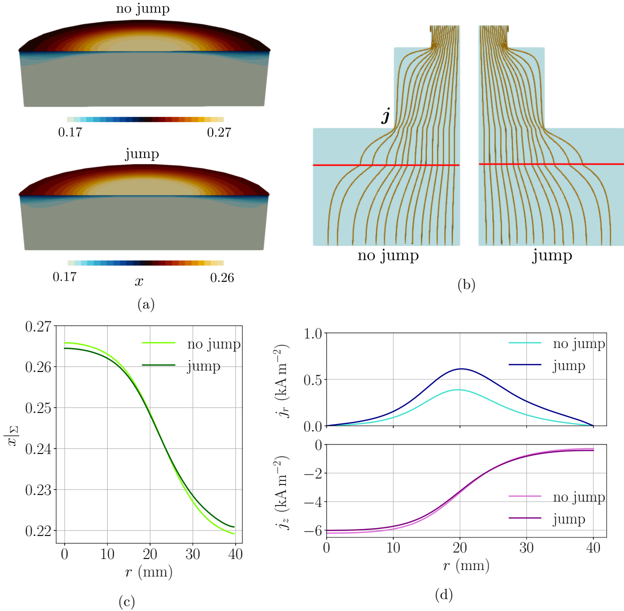
Figure 5.16 – I = 10 A. Molar fraction in the alloy, current density in the case with swirling EVF and buoyancy, at t = 260 s, with or without jump coupling. (a) Snapshots of the molar fraction of lithium in the alloy x . (b) Streamlines of the current density in the cell. (c) Molar fraction x|_{\Sigma} at the alloy-electrolyte interface as a function of radius r . (d) Current density j_r (top) and j_z (bottom) at the alloy-electrolyte interface as a function of radius r .
