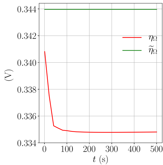
Figure 5.19 – Ohmic losses \eta_{\Omega} and \tilde{\eta}_{\Omega} vs time.
