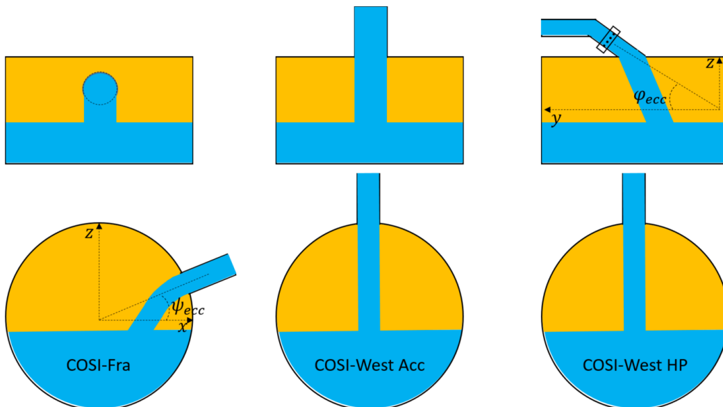
(c) Geometrical configurations of the COSI ECC pipe.
