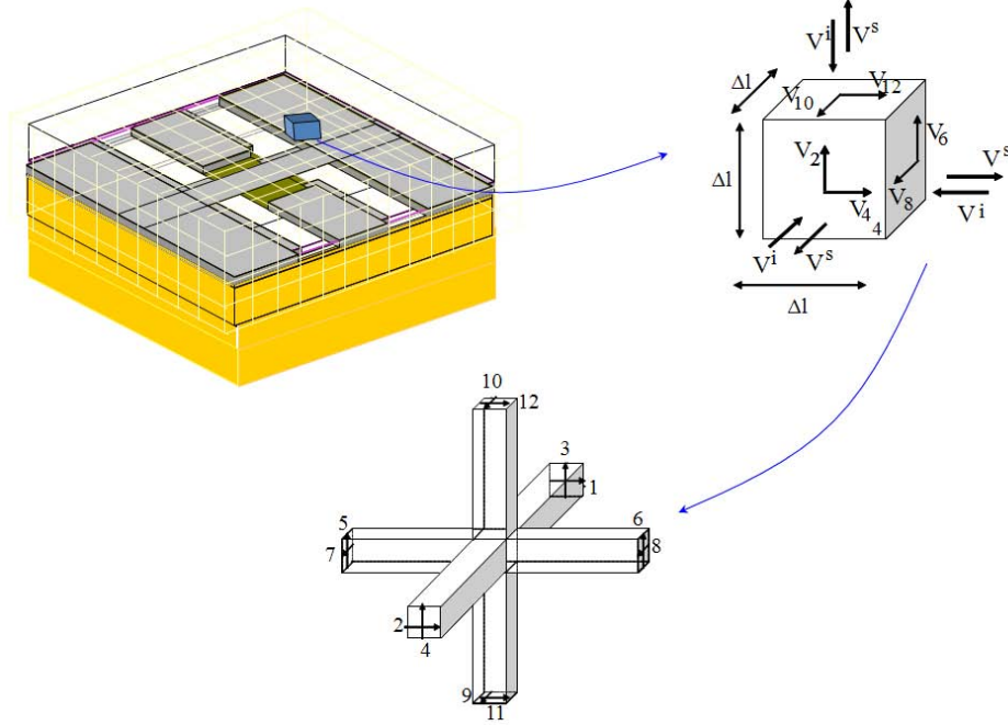
FIGURE 3.3 – Entire space is discretized. On each face of each cell (cuboid) the field is decomposed in the two polarization components ( i stand for incident, s stands for scattered). The cubic cell is modeled by the three-dimensional symmetrical condensed (SCN) TLM node proposed by P. B. Johns in 1986.
