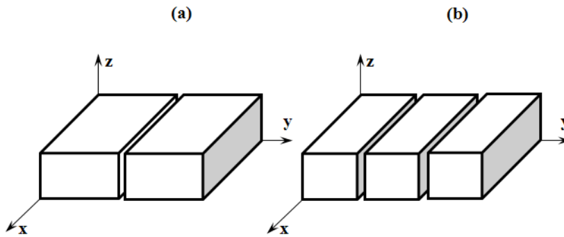
FIGURE 3.9 – Division of the medium to sub-media in one direction on a (a) two and (b) three Grid computing nodes.
