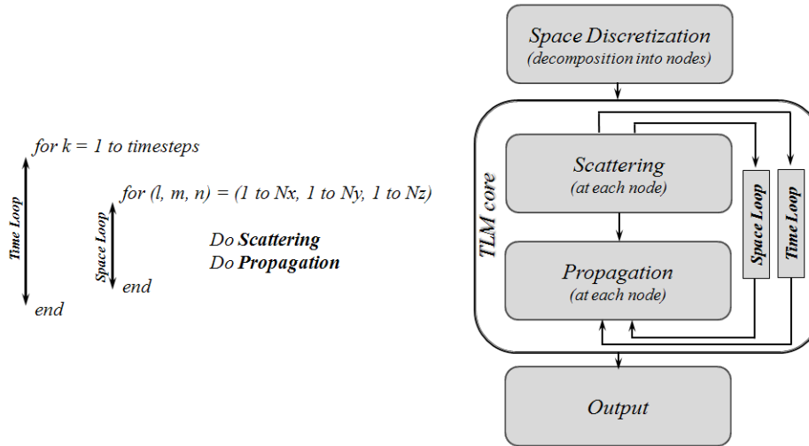
FIGURE 3.4 – TLM Algorithm.
