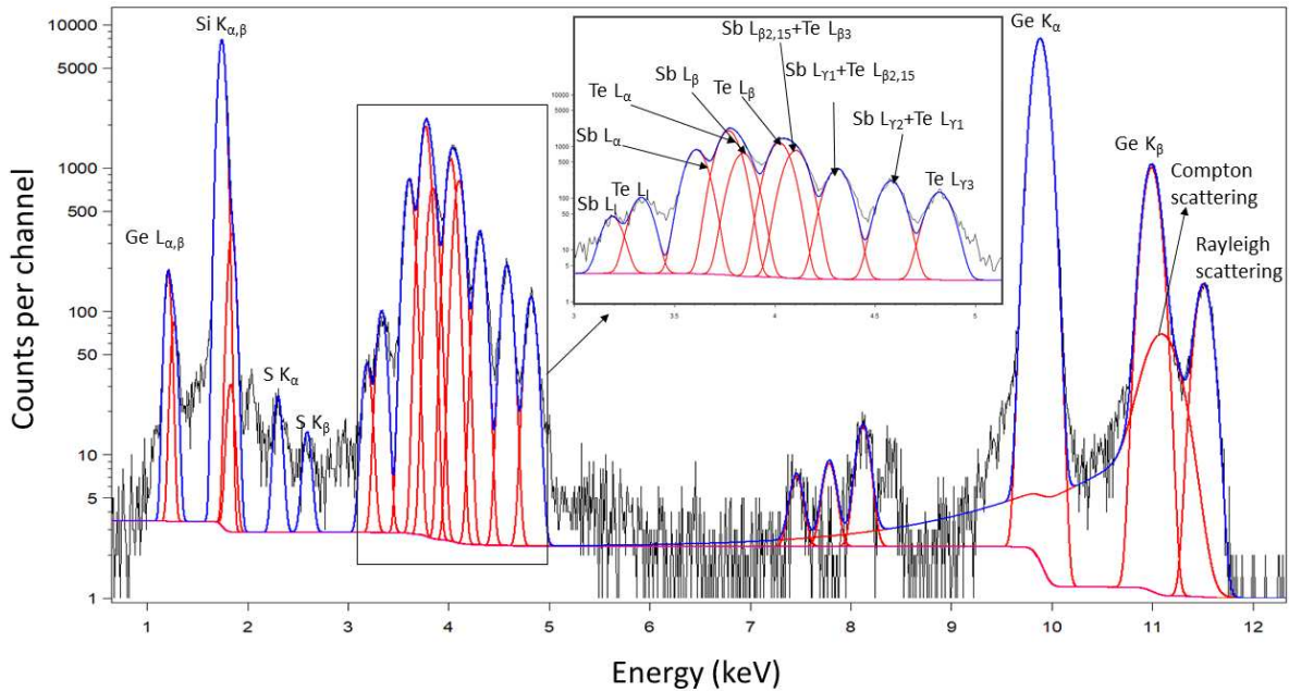
Figure 6.6: X-ray fluorescence spectrum of Te-rich GST acquired at 0.5^\circ incidence with an excitation energy of 11.5 keV and fitted using COLEGRAM.
