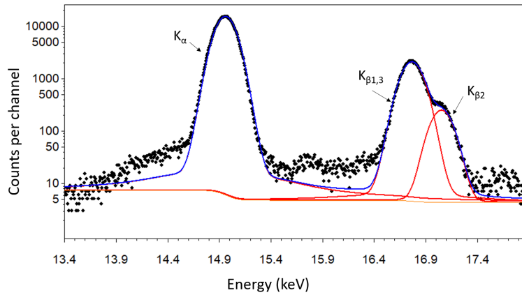
Figure 4.17: Example of Y fluorescence spectrum measured at 25 keV and the processing with COLEGRAM using Voigt functions. The peak at 15.7 represents the Fluorescence Yield measurement K_{\alpha} of zirconium Zr due to contamination.
