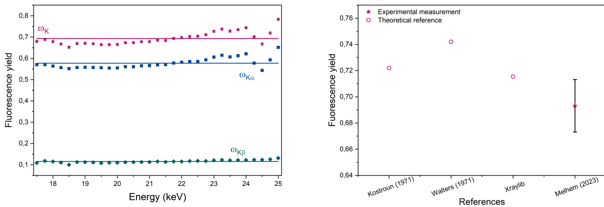
Figure 4.18: Partial and total fluorescence yields of yttrium measured at different incident energies (left) and a comparison of yttrium K - fluorescence yield with reference values (right).
