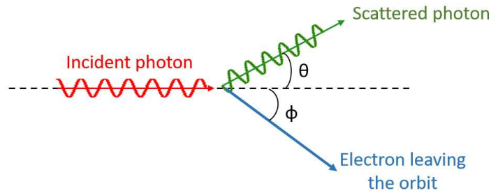
Figure 1.15: Compton scattering; Collision of a photon with an electron at rest and scattering angles.
