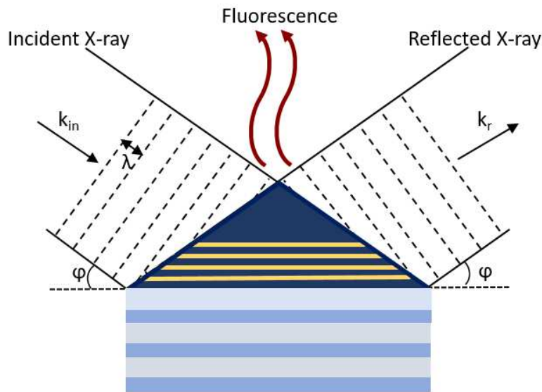
Figure 4.1: A schematic illustration describing formation of an X-ray standing wave (XSW) field under total external reflection of X-rays on a multilayer stack.
