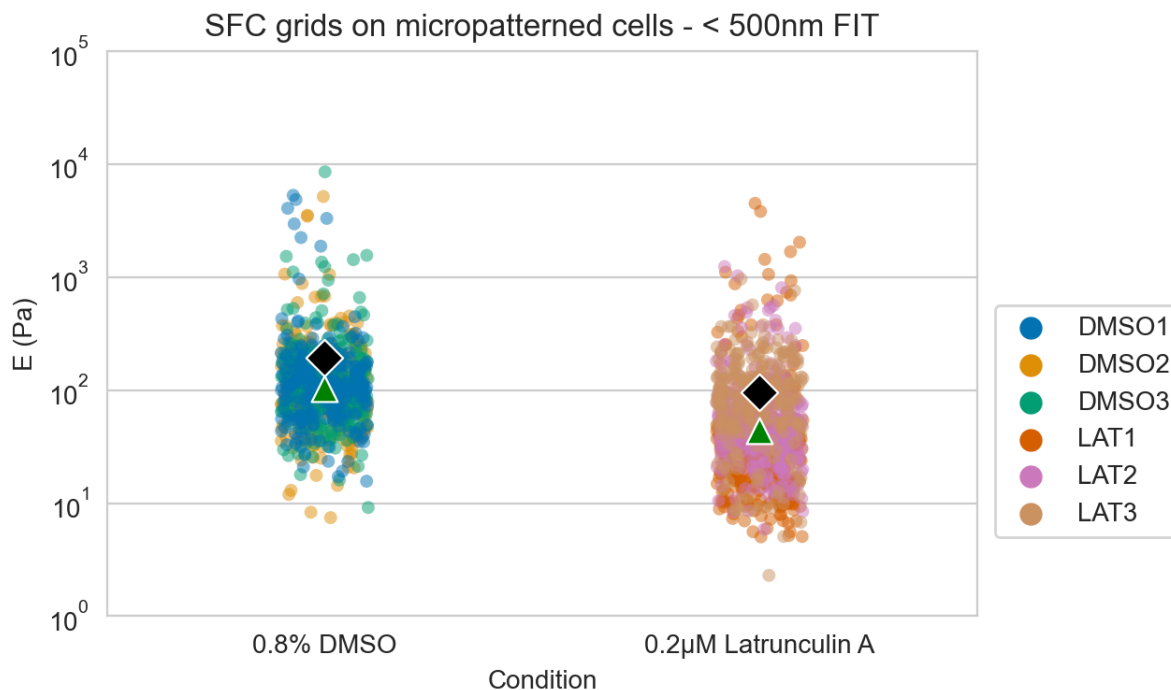
Figure 62: Apparent Young's modulus ( E ) of hTERT-RPE-1 cells seeded on micropatterns. Each point represents the median E of a 4x4 grid of single force curves acquired on the perinuclear region of the cell (0.8% DMSO N = 834 , 0.2 \mu M Latrunculin-A N = 927 ). The black diamond represents the mean (193.38 Pa 0.8% DMSO, 96.22 Pa 0.2 \mu M Latrunculin-A) and the green triangle represents the median (102.47 Pa 0.8% DMSO, 43.64 Pa 0.2 \mu M Latrunculin-A)
