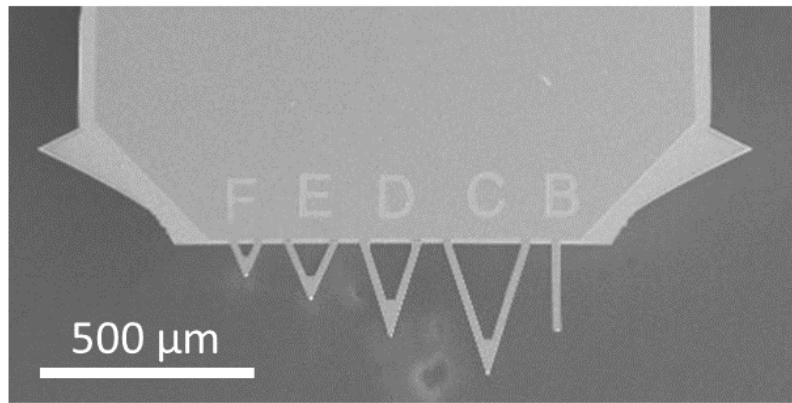
Figure 17: Scanning electron microscope image of a multi-cantilever MLCT-Bio probe. (Courtesy of N. Barois)
