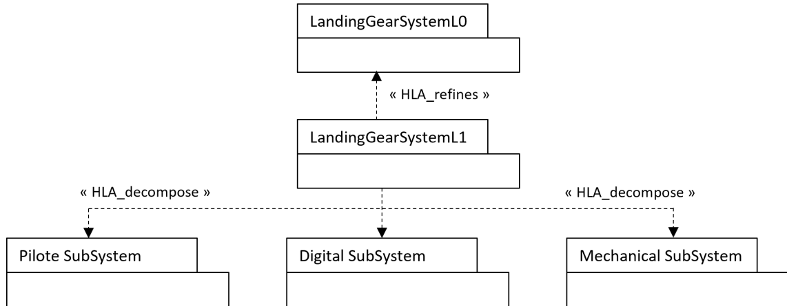
Figure 2.39 – Landing gear system decomposition
