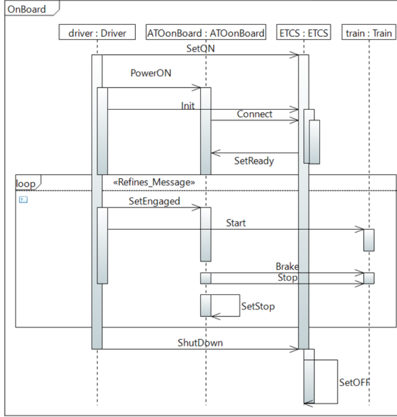
Figure 2.10 – Sequence diagram example
