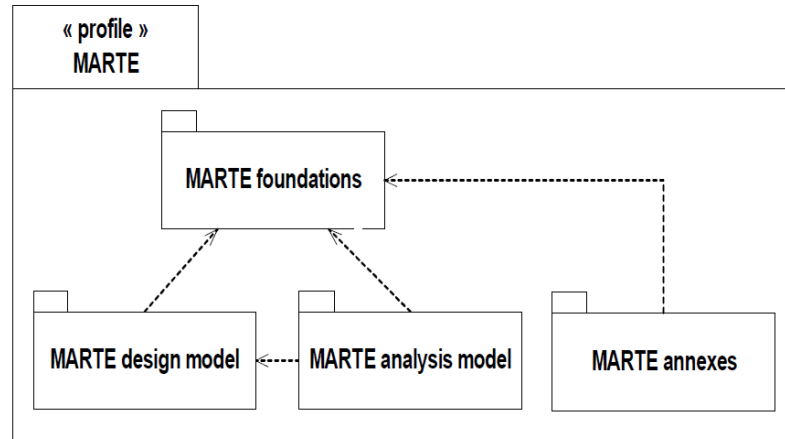
Figure 1.3 – Overall architecture of MARTE
