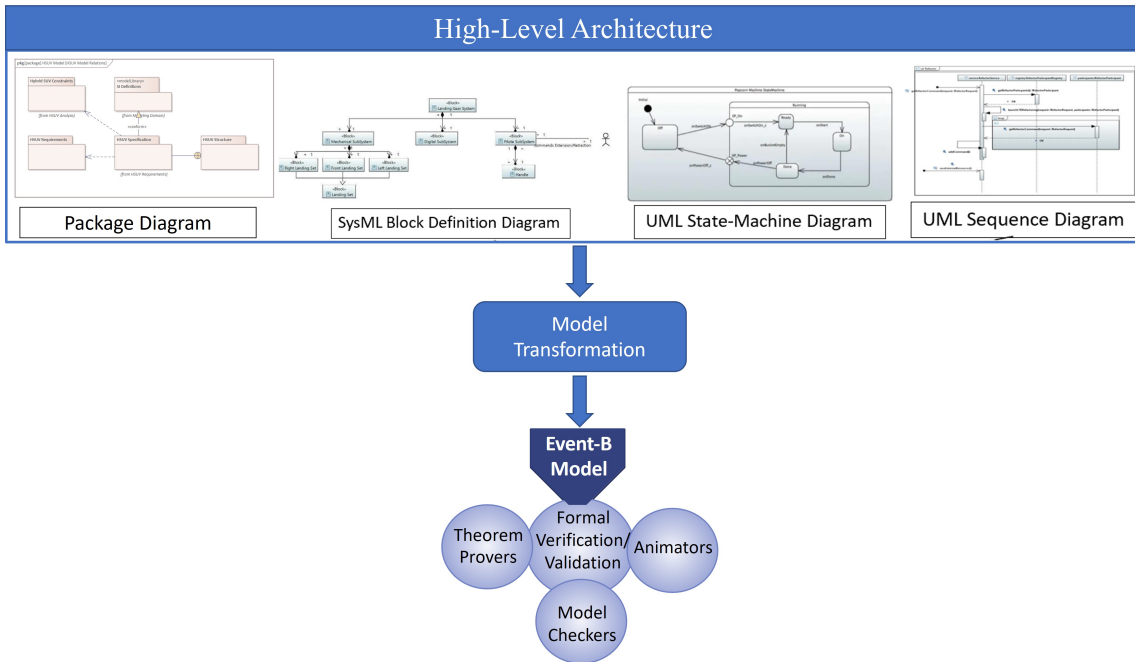
Figure 2.2 – HLA modeling and formalization approach
