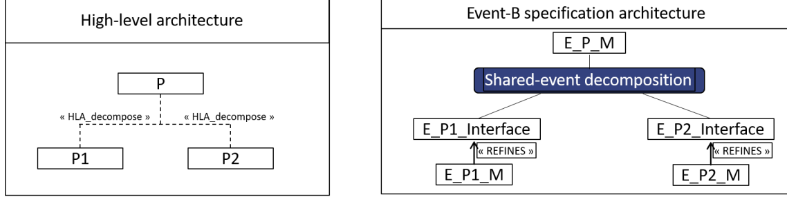
Figure 2.16 – Decomposition extension translation to EVENT-B
