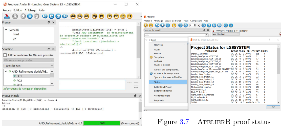
Figure 3.6 – ATELIBB interactive proof tool
