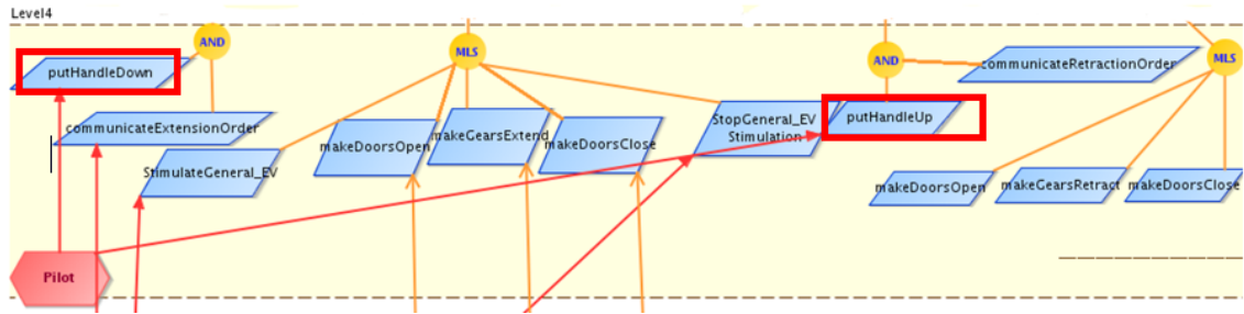
Figure 2.31 – SysML/KAOS PiloteSubSystem assigned goals
