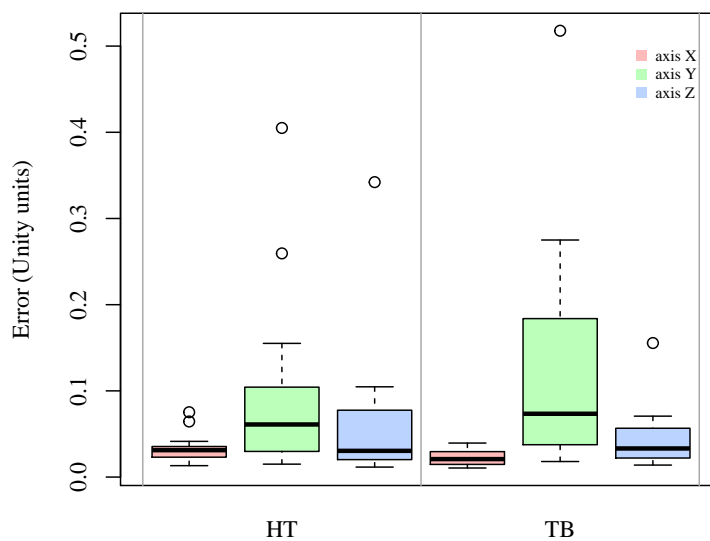
Fig. 3.9 The median value (with inter-quartile range –Q1-Q3) for the analysis of the accuracy measure by axis in the VR prototype for the HT and TB techniques
