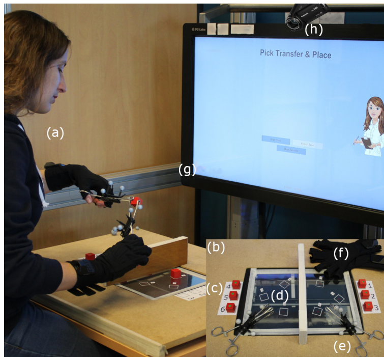
Fig. 4.6 The physical prototype for the PT&P task. (a) User interacting with the system (b) working table composed of the scanner and the wall (c) cubes (d) cubes' targets (e) forceps (f) gloves (g) screen for the instructions (h) recording camera
