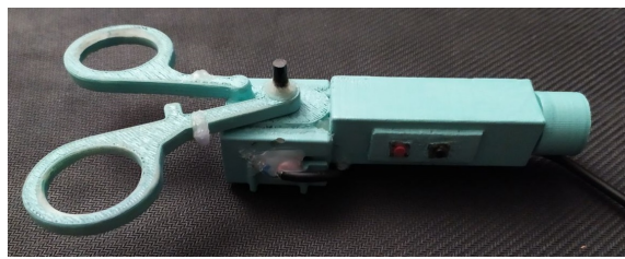
(a) First 3D printed forceps
