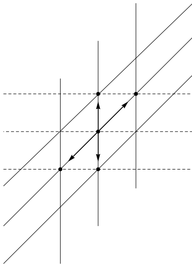
FIG. 3. The deformed square lattice walk steps after the modular transformation.
