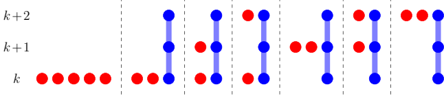
FIG. 11. Seven (1,3)-compositions of 5: (5), (2, 0, 0; 1), (1, 1, 0; 1), (1, 0, 1; 1), (0, 2, 0; 1), (0, 1, 1; 1), (0, 0, 2; 1), illustrated by fermions (red) and three-fermion bound states (blue).
