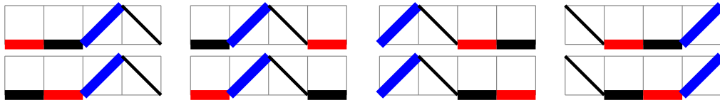
FIG. 4. All the 4c_{1,1,2}(1, 0; 1, 0; 1) = 8 periodic generalized Motzkin paths of length 2n = 4 with \tilde{l}_1 = 1 horizontal step (red), \tilde{l}'_1 = 1 horizontal step of another type (black), and l_1 = 1 up step (blue) originating from the first floor.
