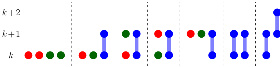
Figure 4.3: Seven (1, 1, 2) -compositions of 4 with \tilde{l}_1 + \dots + \tilde{l}_{j+1} = \tilde{l}'_1 + \dots + \tilde{l}'_{j+1} : (2; 2; 0) , (1, 0; 1, 0; 1) , (1, 0; 0, 1; 1) , (0, 1; 1, 0; 1) , (0, 1; 0, 1; 1) , (0, 0; 0, 0; 2) , (0, 0; 0; 0, 0; 1, 1) , illustrated by two types of fermions (red, green) and two-fermion bound states (blue).
