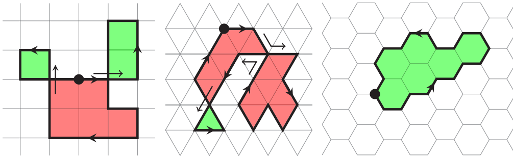
FIG. 1. Closed random walks of length 2n = 20 on the square, triangular, and honeycomb lattice with algebraic area -2 , -12 , and 6 , respectively.
