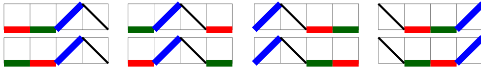
Figure 4.4: All the 4c_{1,1,2}(1, 0; 1, 0; 1) = 8 periodic generalized Motzkin paths of length 2n = 4 with \tilde{l}_1 = 1 horizontal step (red), \tilde{l}'_1 = 1 horizontal step of another type (green), and l_1 = 1 up step (blue) originating from the first floor.
