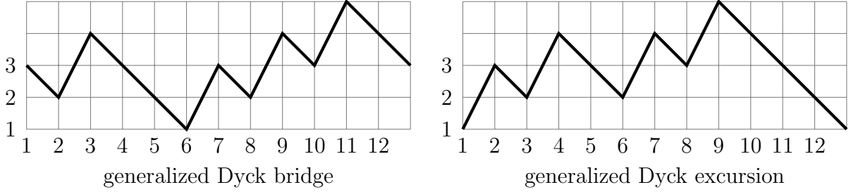
Figure 3.2: A generalized Dyck bridge and a generalized Dyck excursion for g = 3 , which starts from the third floor and the first floor, respectively, of length \mathbf{n} = 12 with l_1 = 1 up step from the first floor, l_2 = 2 up steps from the second floor, and l_3 = 1 up step from the third floor. We refer to them as periodic generalized Dyck paths.
