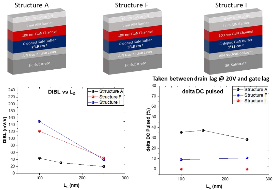
Figure.3.15. DIBL (left) and delta DC pulsed taken between drain lag at V_{DS}=20\text{V} and gate lag (right) as a function of different gate lengths for each structure.
