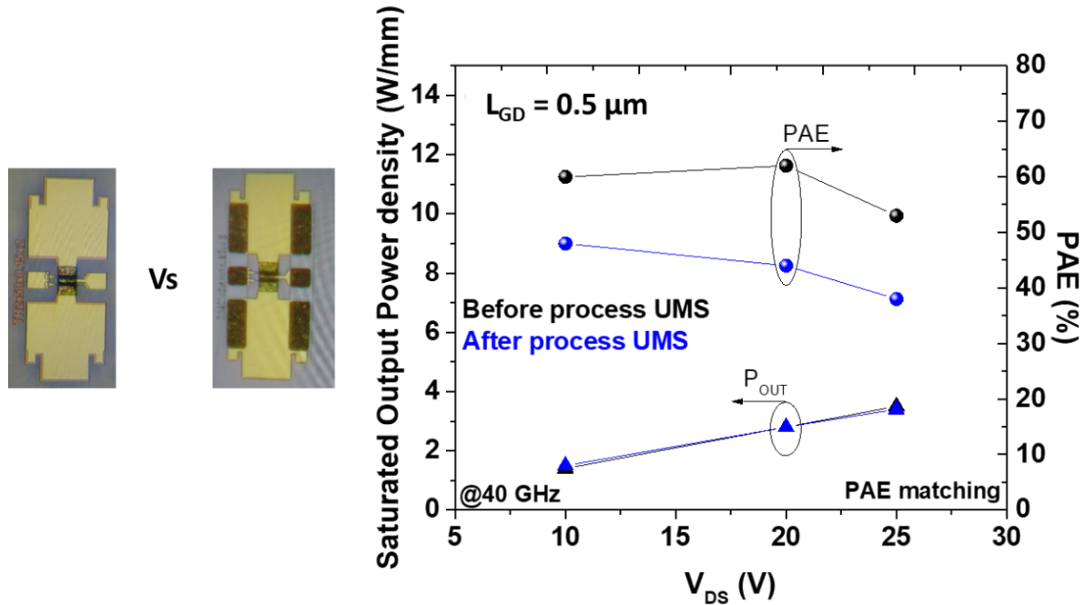
Figure.3.68. PAE and output power density ( P_{OUT} ) as a function of V_{DS} in CW mode of 2 \times 50 \mu m IEMN PCMs with L_G = 105 \text{ nm} and L_{GD} = 0.5 \mu m before and after UMS processing
