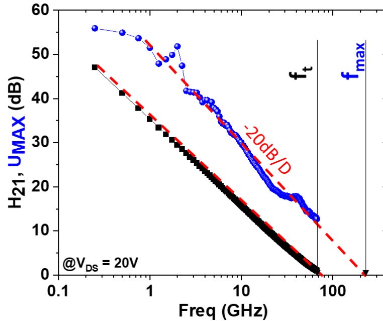
Figure.2.27. An example of U and H_{21} curves used for the extraction of f_t and f_{max}
