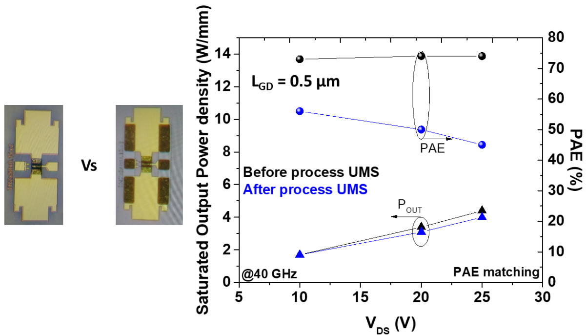
Figure.3.69. PAE and output power density ( P_{OUT} ) as a function of V_{DS} in pulsed mode of 2 \times 50 \mu m IEMN PCMs with L_G = 105 \text{ nm} and L_{GD} = 0.5 \mu m before and after UMS processing
