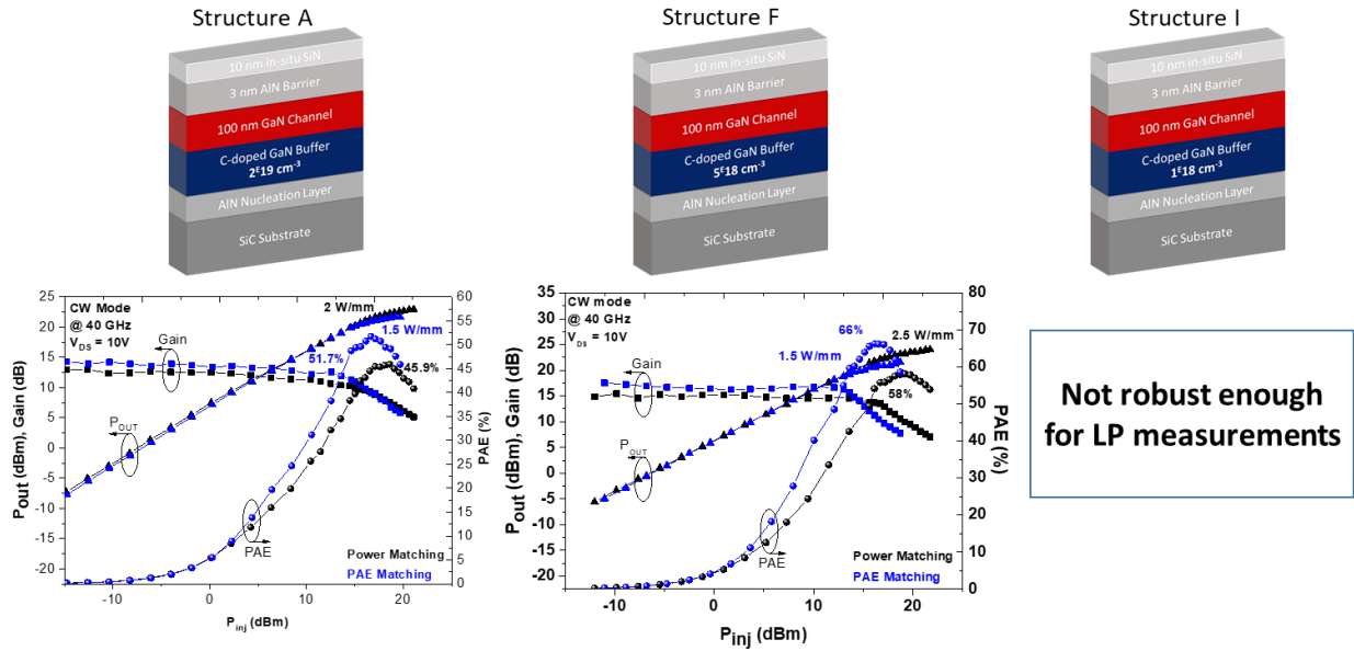
Figure.3.14. Load-pull measurements at 40 GHz and V_{DS} = 10\text{V} of the structures with a C-doping buffer variation
