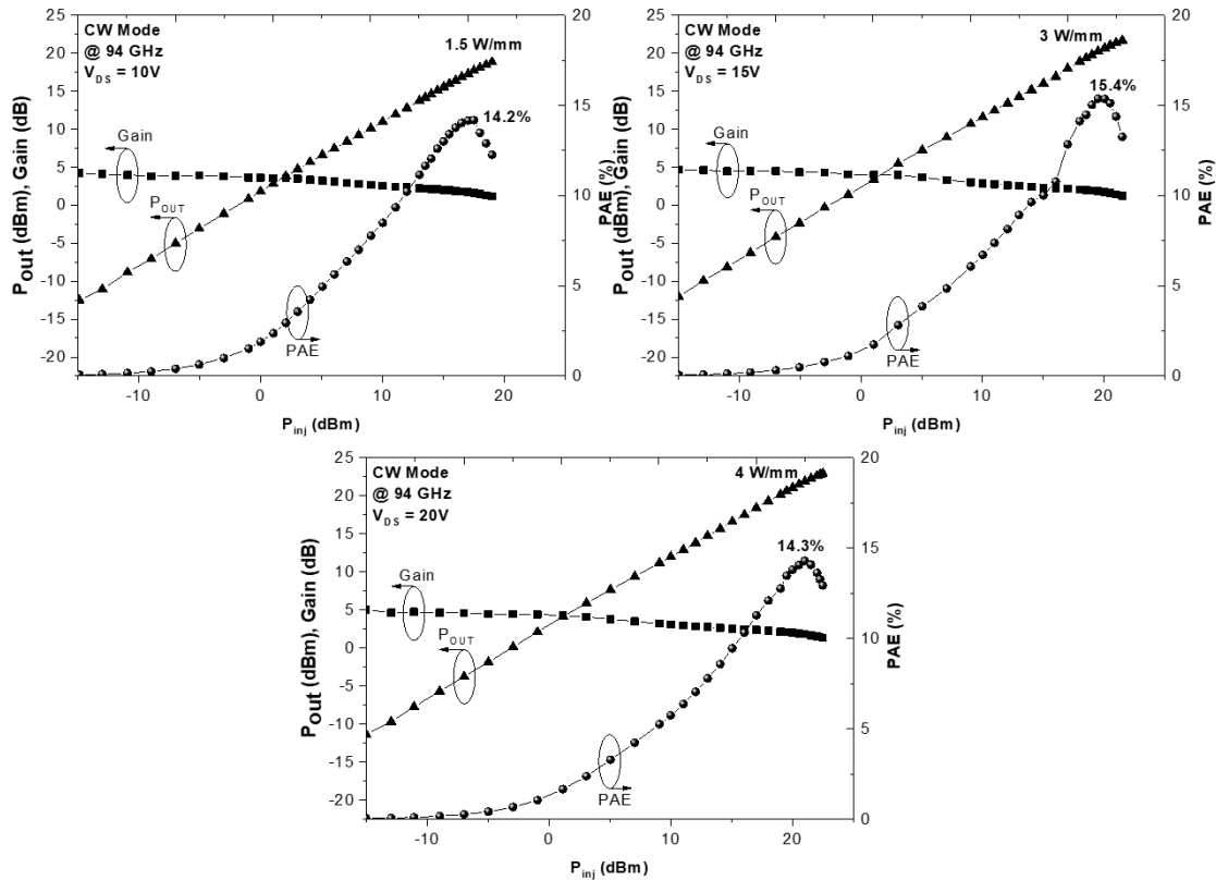
Figure.3.73. CW large signal performances at 94 GHz for 2 \times 25 \mu\text{m} transistor L_G = 105 \text{ nm} and L_{\text{GD}} = 0.5 \mu\text{m} at V_{\text{DS}} = 10, 15, and 20\text{V} of the 3 nm AlN/GaN HEMT structure
