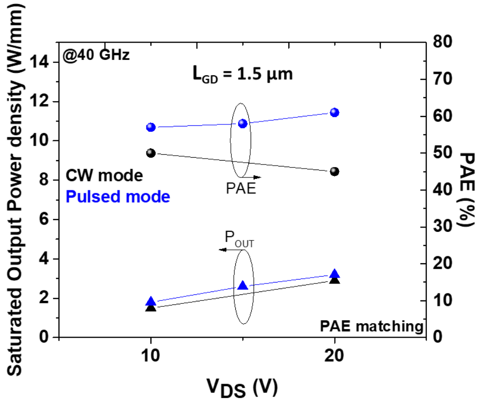
Figure.3.32. PAE and output power density ( P_{OUT} ) vs V_{DS} in pulsed and CW mode of the 4 nm AlN/GaN HEMT structure.
