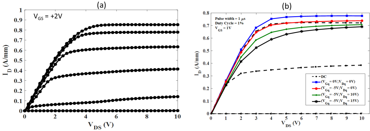
Figure.4.23. I-V (a) and pulsed I-V (b) characteristics of a 2 \times 50 \mu m transistor with L_G = 100 nm and L_{GD} = 1.5 \mu m of the 14 nm AlGaIn/GaN buffer-free structure.
