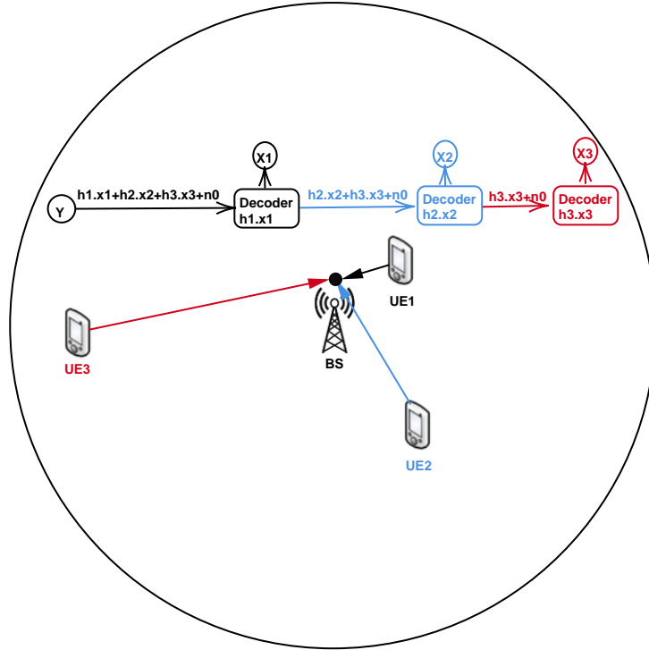
Figure 2.11: NOMA Uplink
