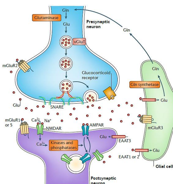
Figure 34. Transmission synaptique glutamatergique (Popoli et al., 2012)
