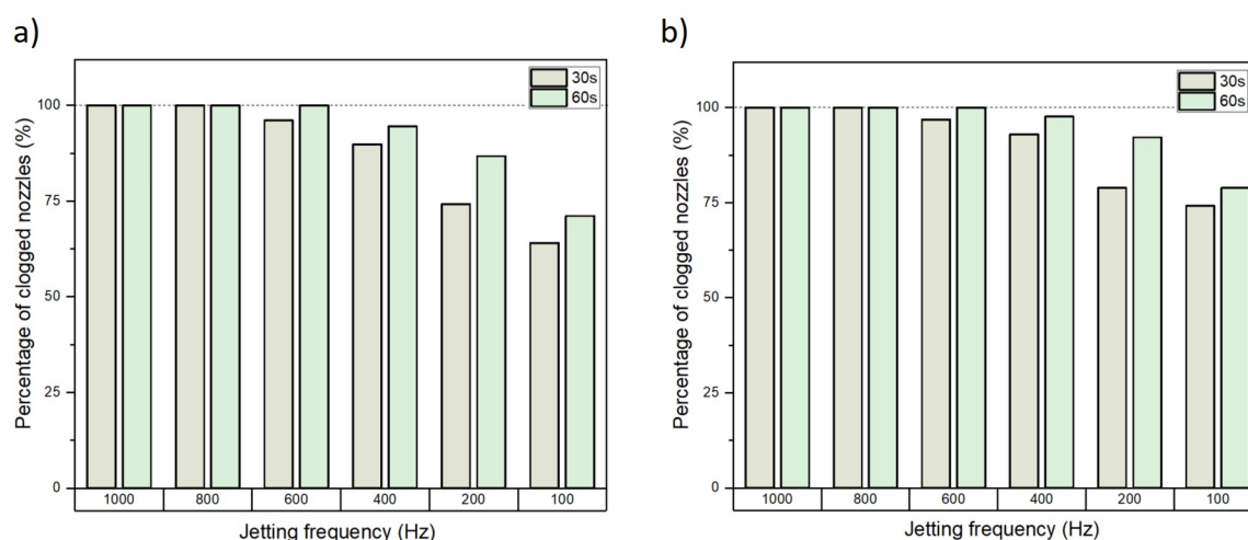
Figure 4.13: The percentage of clogged nozzles after 30 and 60s of ejection as a function of jetting frequency for anode inks: a) INK_SiOC_CMC; b) INK_SiOC_PEDOT.
