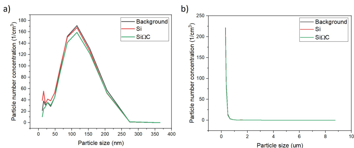
Figure 4.22: The particle number concentrations per \text{cm}^3 during anode ink formulation for: a) nanoparticles, b) microparticles.
