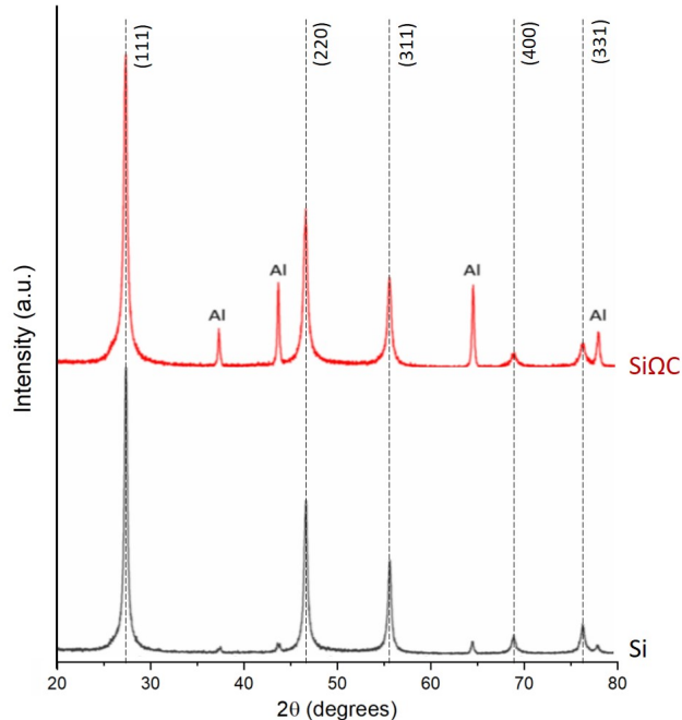
Figure 2.21: XRD patterns of Si and \text{Si}\Omega\text{C} nanoparticles.
