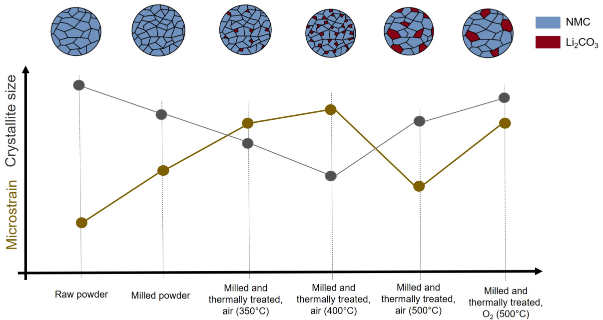
Figure 3.15: Schematic representation of changes in crystal structure induced by high-energy ball milling and thermal treatment.
