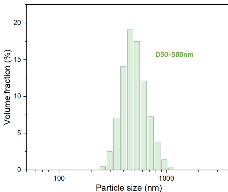
Figure 2.25: Particle size distribution of Super P Carbon Black measured using Zetasizer Nano ZS.
