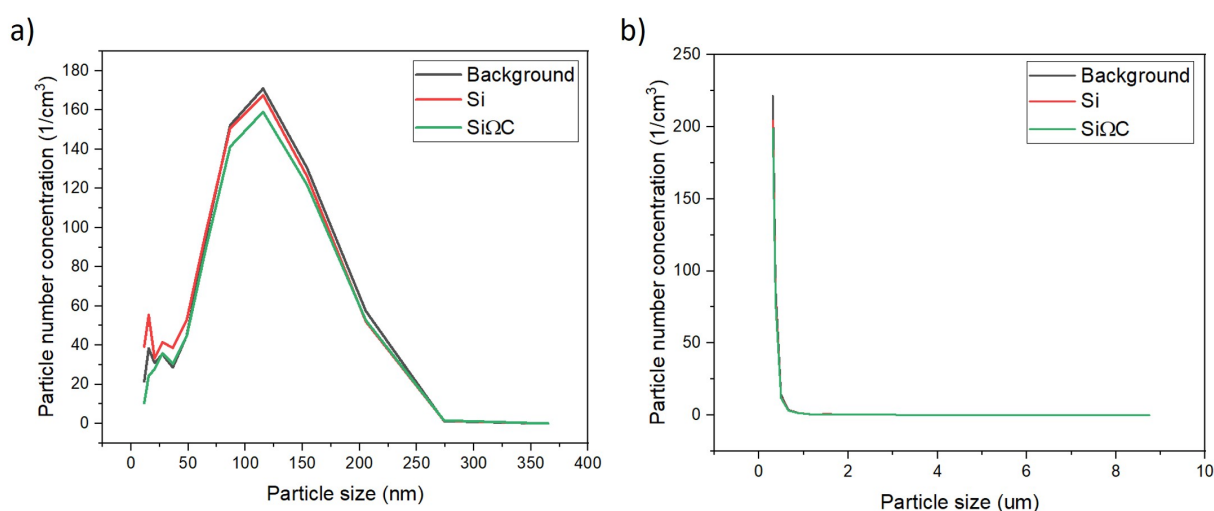
Figure 4.22: The particle number concentrations per cm 3 during anode ink formulation for: a) nanoparticles, b) microparticles.
