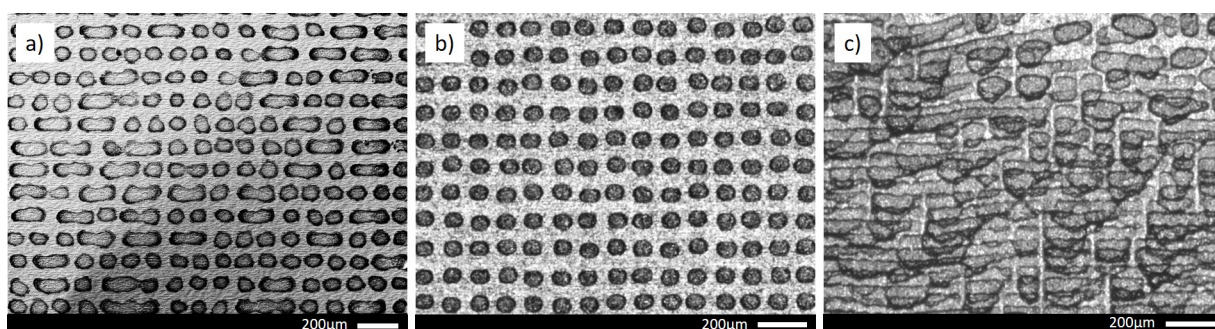
Figure 4.21: Single splats of INK_Si \Omega C_CMC: a) without heating of the substrate, b) with the substrate temperature of 50°C, c) after 3 passes of printing with the substrate temperature of 50°C.
