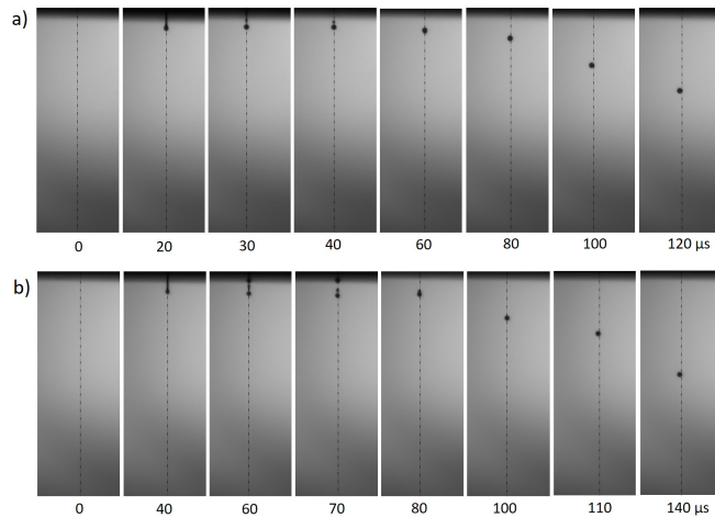
Figure 4.10: Drop generation process with optimal parameters registered as a function of time for: a) INK_SiΩC_CMC; b) INK_SiΩC_PEDOT.
