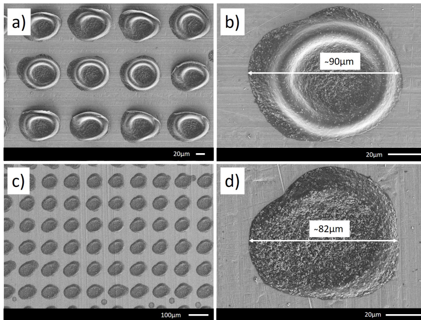
Figure 5.20: SEM observations of deposited 3D structures with INK_CMC: a) pillars deposited with the substrate holder temperature of 40°C, b) single pillar deposited with the substrate holder temperature of 40°C, c) pillars deposited with the substrate holder temperature of 60°C, d) single pillar deposited with the substrate holder temperature of 60°C.
