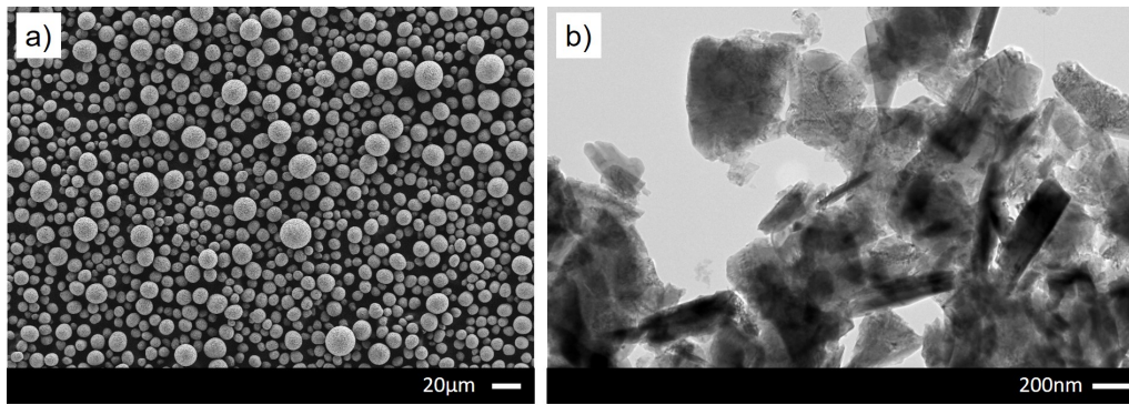
Figure 3.4: a) SEM image of raw NMC622 powder, b) TEM image of high energy ball-milled NMC622 powder.
