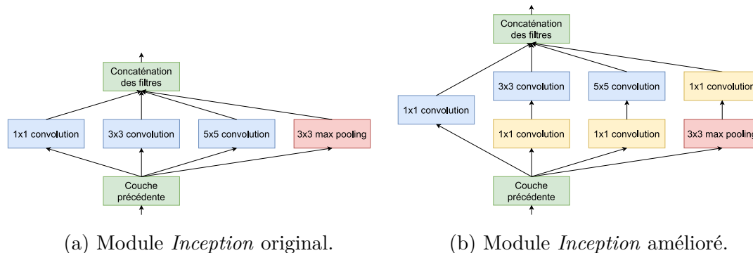
FIGURE 1.5 – Modules Inception .
