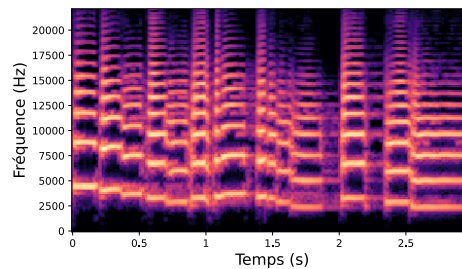
(f) Mel-Spectrograme.
