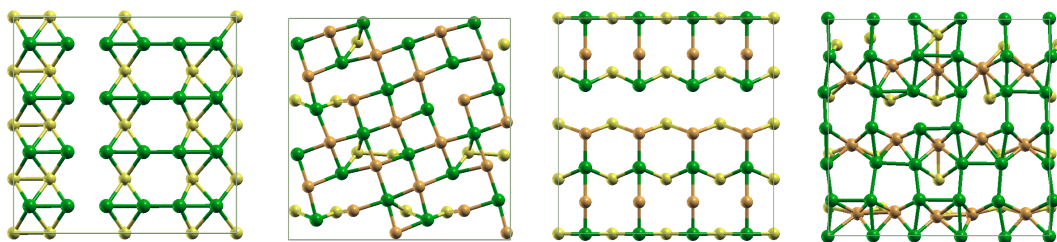
Figure 23: Interface structures before and after energy minimization. On top, the top view of the stacking of the different non-relaxed interfaces. Only the bottom silicide layer and the top silicon layer are shown. On the bottom, top and side view of the relaxed interfaces. Only interface regions are shown. Si atoms belonging to the silicon and silicide slabs are shown in yellow and orange, respectively. Ni atoms are shown in green.
