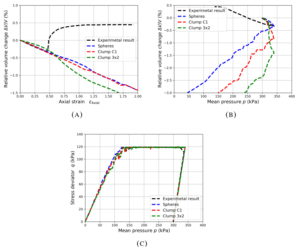
FIGURE 3.16: Validation on constant stress deviator loading paths on loose Hostun sand, comparison with experimental test with q = 119 kPa.
