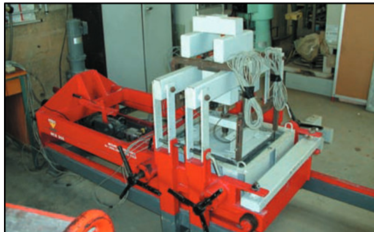
FIGURE 5.4: The direct shear test (Reiffsteck et al., 2007)
