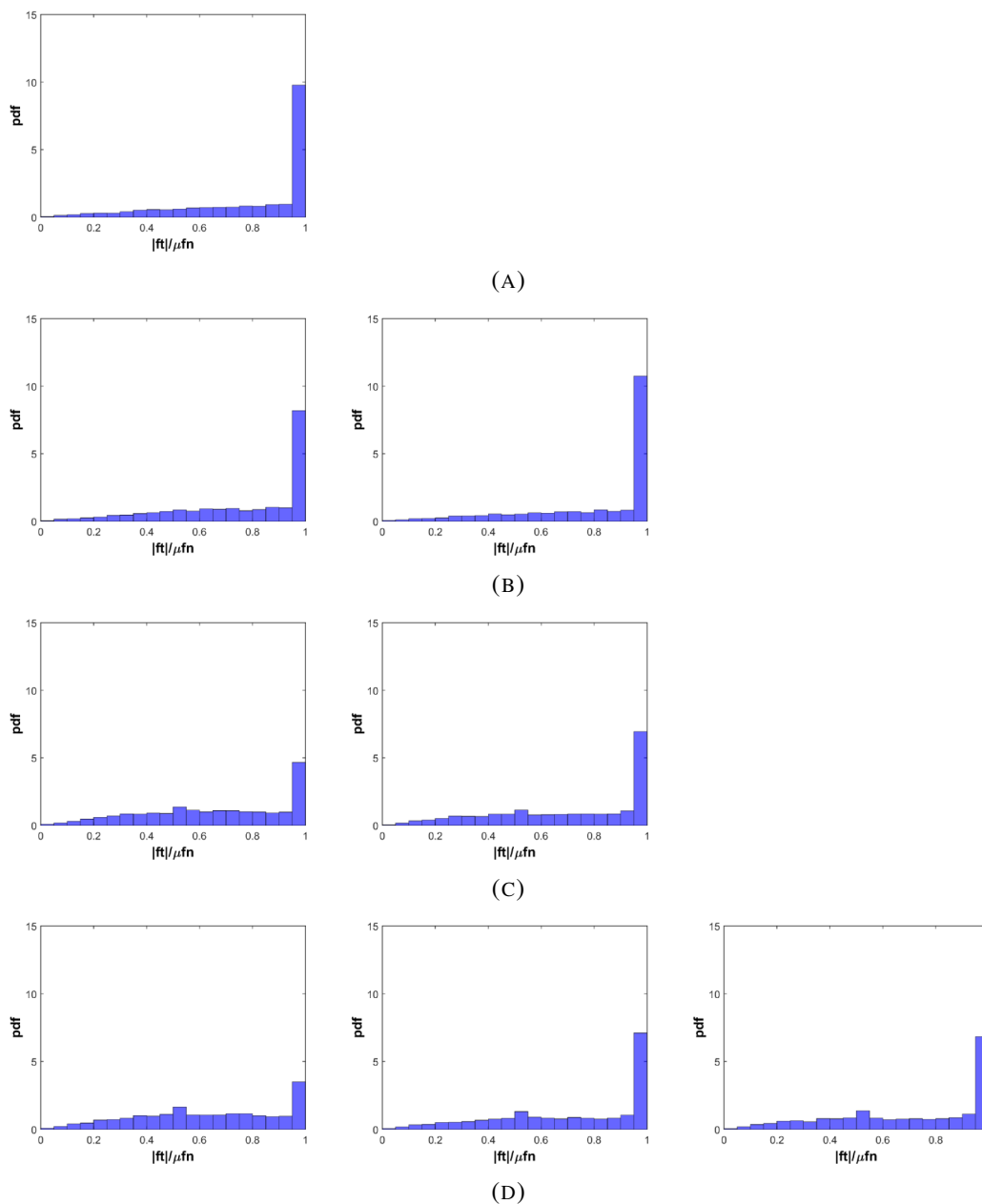
FIGURE 3.36: Probability distribution function of the mobilized friction angle of weak forces. (a) Isotropic model - constant friction angle (b) Anisotropic model - constant friction angle. (c) Isotropic model - non constant friction angle. (d) Anisotropic model - non constant friction angle.
