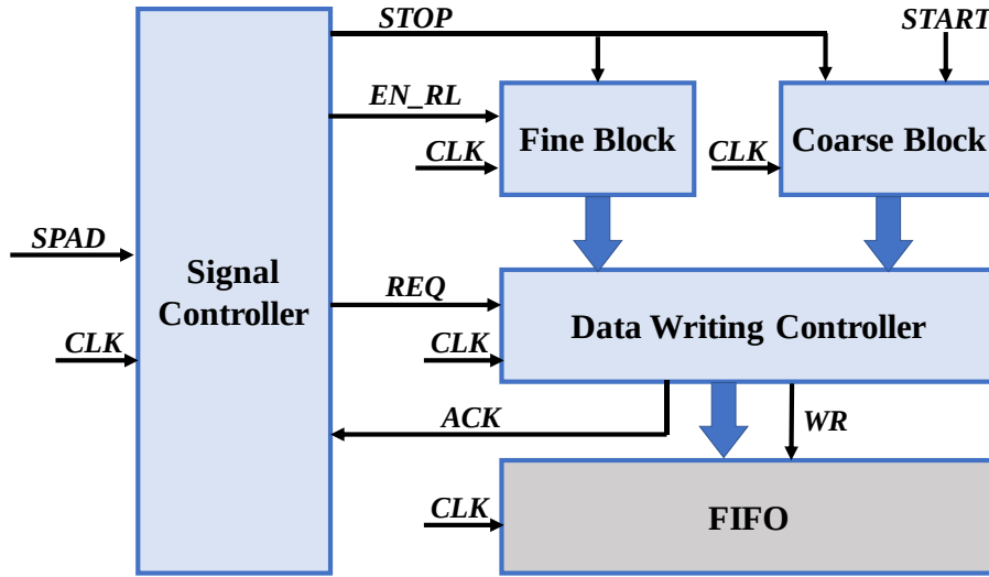
Figure 3.2 Global architecture of the synchronous TDC.
