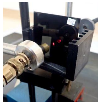
Figure 7.22 Simulating different levels of biofouling by inserting optical attenuators with different optical densities between the laser diode and the SPAD.
