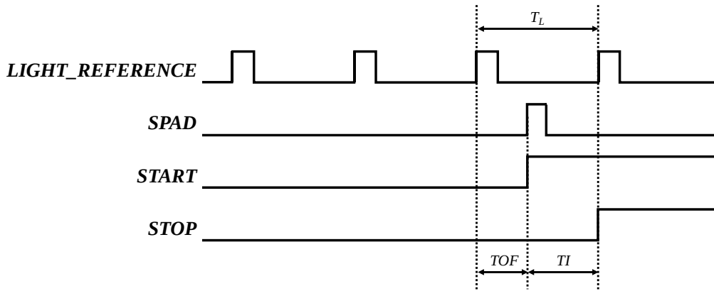
Figure 3.26 Revers start-stop mode: the SPAD signal represents the START signal and the excitation light reference represents the STOP signal, TOF is calculated by subtracting the measured time interval from the excitation light period.
