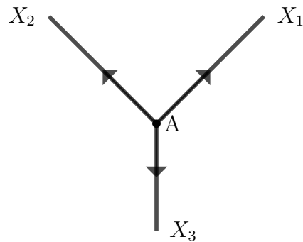
Figure 3.1: The space obtained by gluing X_1 , X_2 and X_3 along A .
