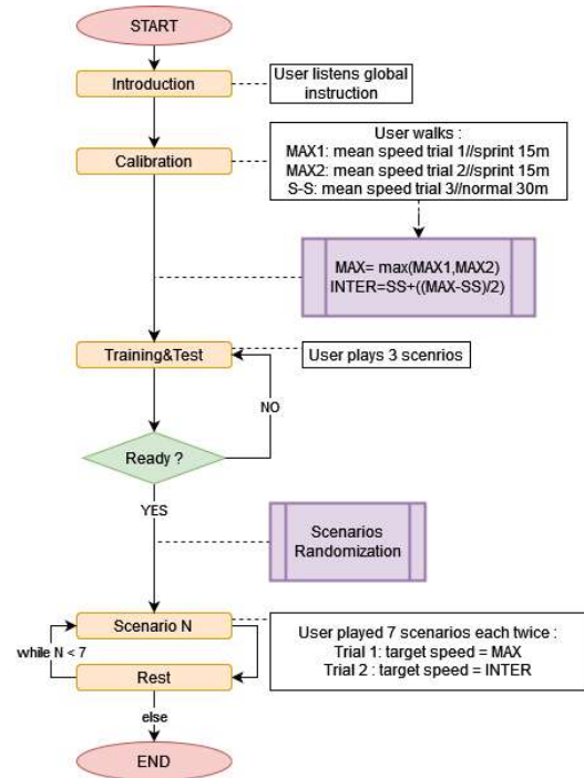
Fig. 1. Software Flowchart. The application started with a welcome message showing the holographic environment. The aim of the clinical study was explained to the patient through oral instruction.. Then, the calibration scene consisted of 2 \times 15 m walking sprints at maximal speed and 1 \times 30 m walking trial at self-selected speed, with no feedback except startup vocal instruction. The calibration gave 2 values that used as individualized target speed for the patient: MAX-the maximal walking speed and INTER-the intermediate walking speed. Three mini-games were then played for the warm-up and adaptation with the system and the holograms. When he/she was ready, the child decided to start the clinical study. The first scenario was displayed in random order. Each trial consisted of walking on 30 m in a straight line at the target speed (MAX and INTER), with one of the 6 scenarios including different feedback characteristics or without feedback (control). Each trial was followed by a rest period.
