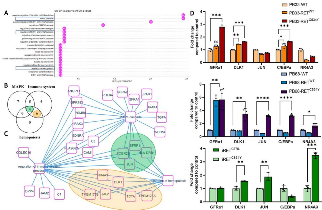
Figure 5. MAPK cascade overlaps the immune system and hemopoiesis network induced by RET C634Y mutation in hematopoietic cells derived from iPSCs. (A) Bar plot of functional enrichment performed on GO-BP database with the 109 coding genes found upregulated in iRET C634Y hematopoietic cells. (B) Venn diagram for overlapping of MAPK, immune system, hemopoiesis gene sets upregulated by RET C634Y mutation. (C) MAPK and hemopoiesis regulation molecular network activated by RET C634Y . (D) Expression of RET-regulated candidate genes quantified by qRT-PCR in iPSCs-derived hematopoietic cells after 13 days of differentiation. Experiments have been performed 3 times. P-values were calculated using a 2-tailed Student's t-test. ns, not significant; *, P < 0.05; **, P < 0.01; ***, P < 0.001; ****, P < 0.0001.
