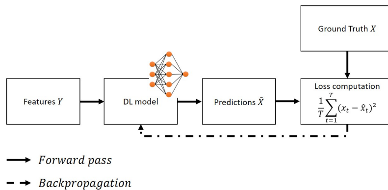
Figure 1.7. One training iteration representation; forward pass and backpropagation alternation
