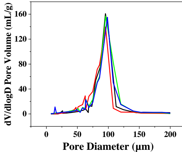
Figure 5. The diameter and volume of different PAAM hydrogel having the same composition and preparation technique
