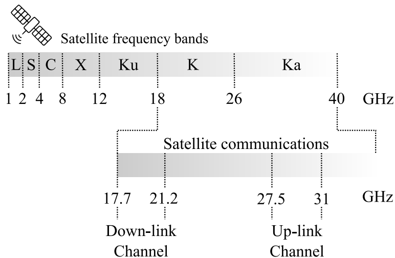
FIGURE 1.3: Frequency allocation of modern SatCom links for both civil and military applications.
