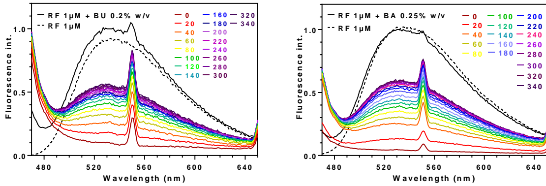
Figure II.S3. Fluorescence emission spectra of riboflavin (RF) migrating from the supernatant to the hydrogels. At t_0 , the supernatant contained RF 2 \mu\text{M} in PBS. Each spectrum was acquired every 20 minutes and normalized by the emission spectrum of the hydrogel + RF 1 \mu\text{M} .
