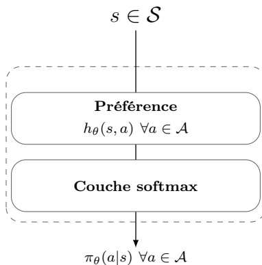
FIGURE 10.3 – REINFORCE profond
