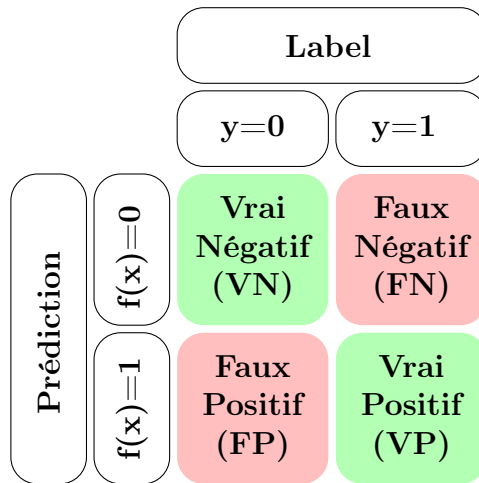
FIGURE 1.3 – Matrice de confusion
