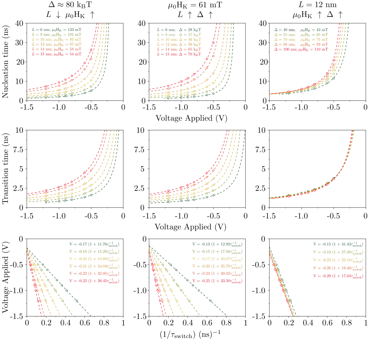
Figure 2.14: Dependence of the nucleation time (ns), transition time (ns) and the inverse of the switching time on the applied voltage, for a situation of a fixed \Delta , fixed L and fixed \mu_0 H_{\text{eff}}^{\text{K}} .
