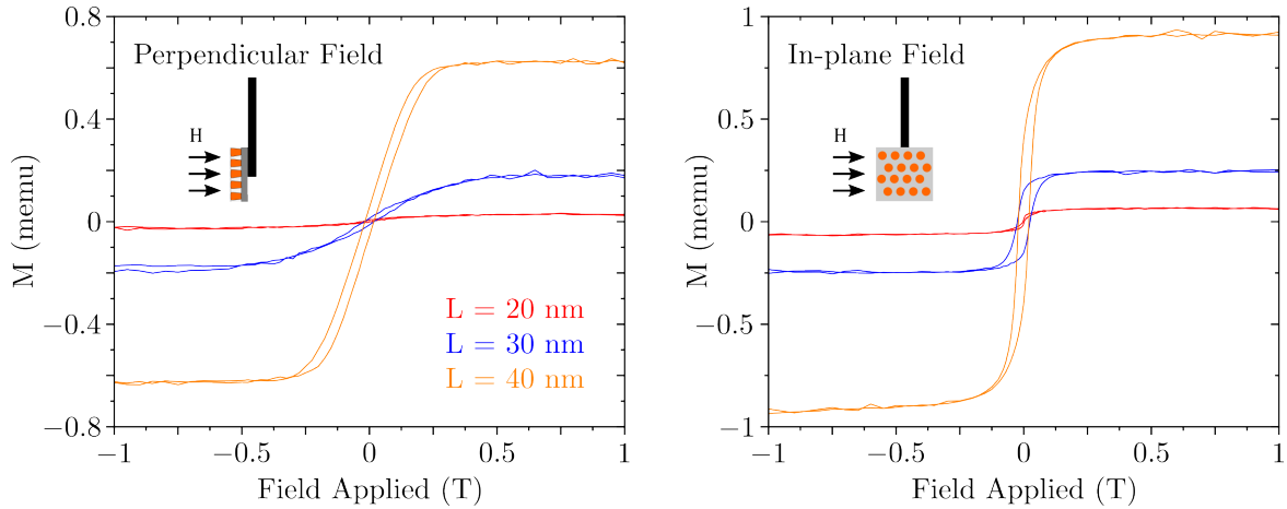
Figure 4.13: Vibrating sample magnetometry in perpendicular and in-plane configuration for a sample with magnetic vias with a height of 20, 30 and 40 nm.
