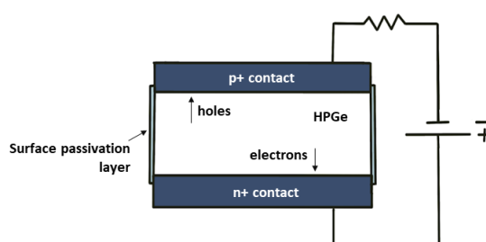
Figure 1.7: HPGe detector technique representation.
