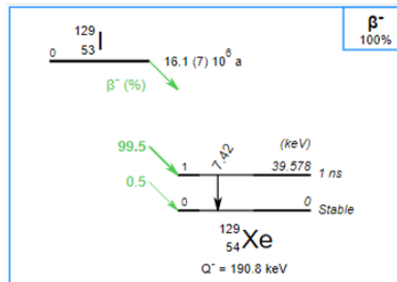
Figure 4.21: The decay scheme of ^{129}\text{I} [35].
