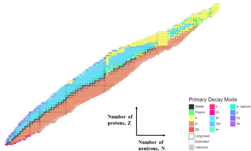
Figure 1.1: Nuclide chart [12].
