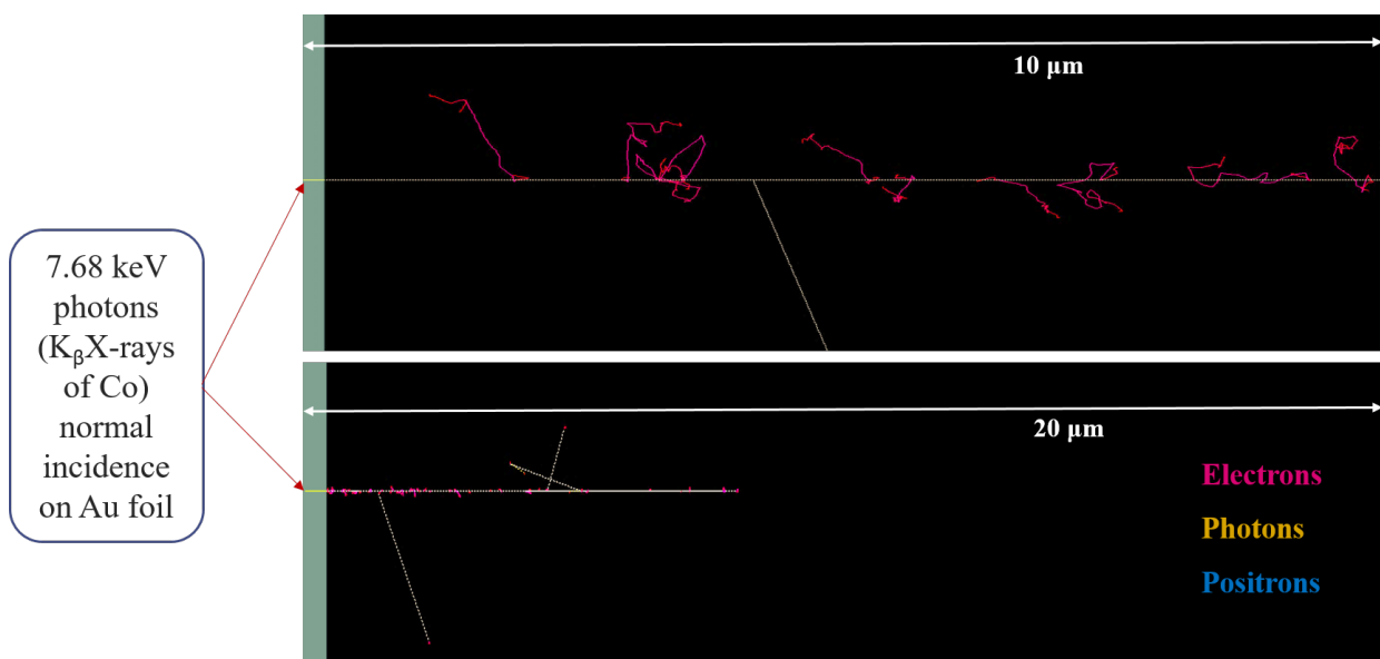
Figure 3.4: Monte-Carlo simulated showers for 59 Ni.
