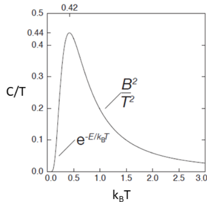
Figure 2.5: Schottky anomaly of the heat capacity for a two-level system.
