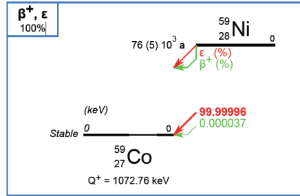
Figure 3.15: Decay scheme of ^{59}\text{Ni} [35].
