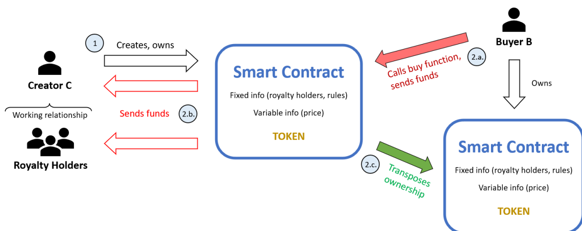
Figure 35: Overview of the advanced Token Level Smart Contract (TLSC). Numbers represent steps, in order; white arrows show ownership; red arrows show purchase execution; white and red arrows show royalty distribution; green arrows show changing of hands of the TLSC.
