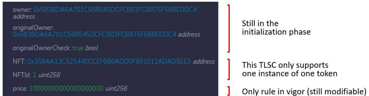
Figure 53: Owner and token-related variable states of a Token Level Smart Contract (TLSC) after an Ethereum test scenario initialization.
