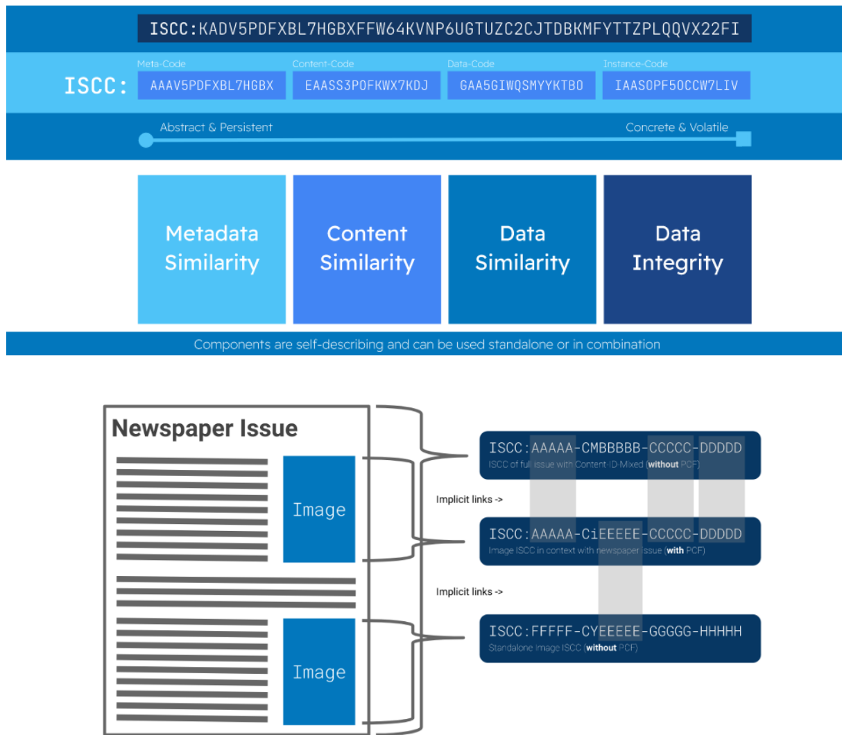
Figure 72: Basic structure of the International Standard Content Code [ISC23b] (left) and illustration of its content flagging.
