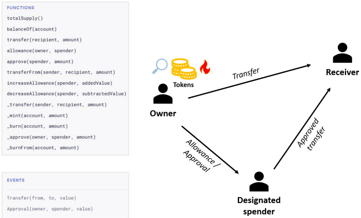
Figure 13: ERC20 Ethereum fungible token standard functions and events [OP223b] (left) followed by an illustration of the roles and actions defined by the standard (right).
