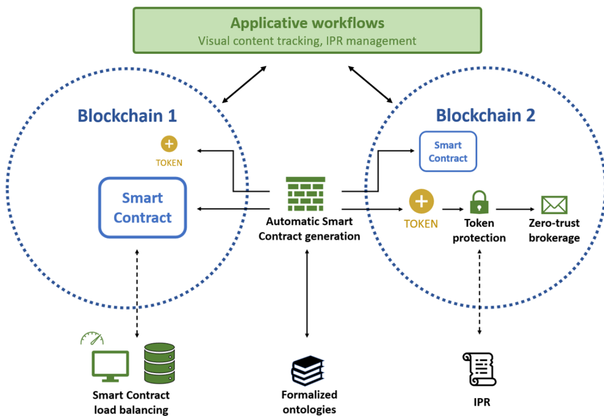
Figure 83: Overview of how the solutions brought forth in this thesis (shown in green) address the applicative blockchain critical limitations identified in our state-of-the-art analysis and summarized in Figure 1. Token-centered solutions were brought forth to enable their protected distribution and persistent Intellectual Property Right links with underlying assets (shown in Blockchain 2). Smart Contract limitations were also tackled by enabling their systematic generation across blockchains and the processing of prior prohibitively complex operations (shown in the center and in Blockchain 1, respectively). Each of these solutions was also built to interoperate with others and further versatile applicative workflows.
