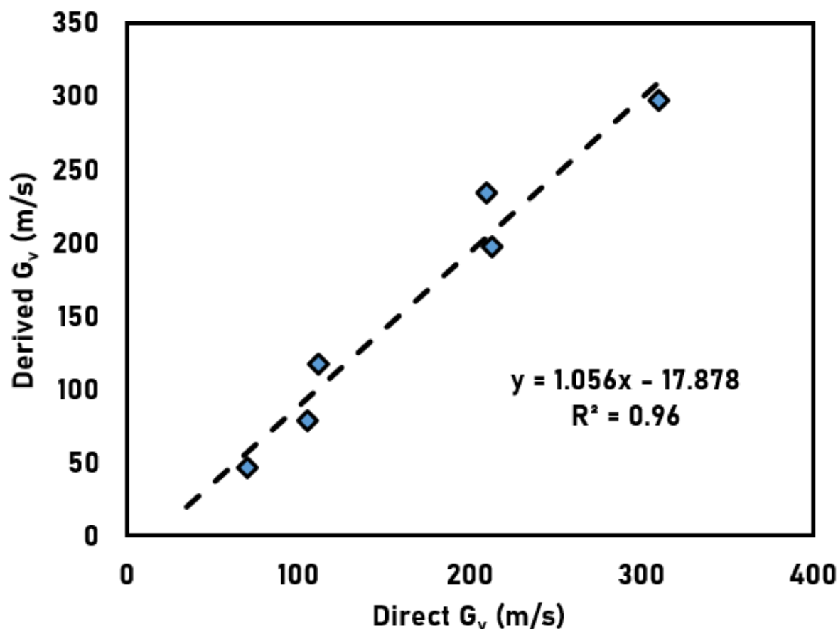
Fig. 4-1 Comparison between max gas velocity ( G_v ), as derived from ballistic ejection velocity, and directly measured maximum gas velocities for major to paroxysmal eruptions at Stromboli. See Table 4-1 for data and sources.
