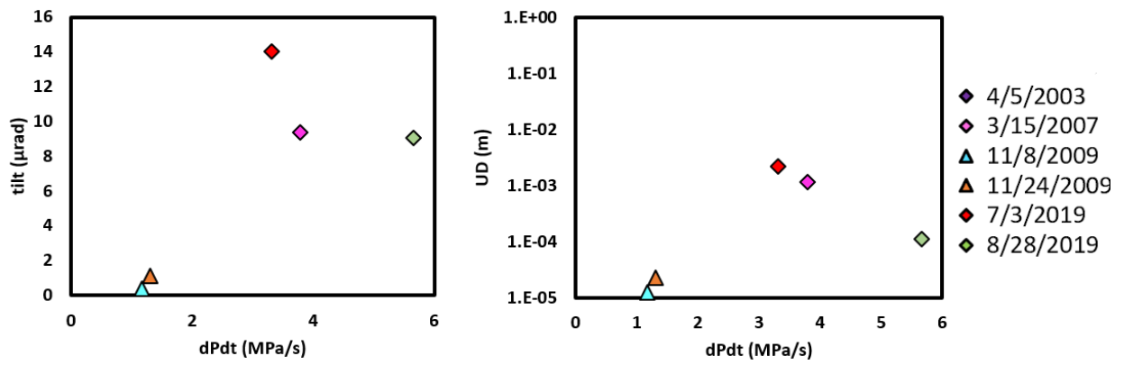
Figure S3-12: Embayment-driven maximum decompression rate vs surface tilt (left) and seismic amplitude (right). Triangles and diamond are for major and paroxysmal eruptions, respectively. No trend can be seen from either of these plots.
