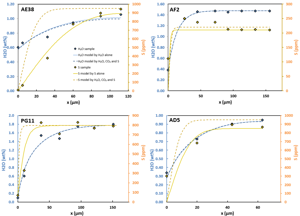
Figure s2-16: Best fit diffusion profiles calculated from EMBER on Ambrym data from Moussallam et al. [2021]
