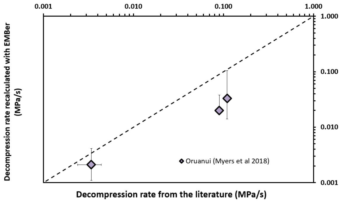
Figure s2-13: Comparison between decompression rate from original study and those recalculated by EMBER
