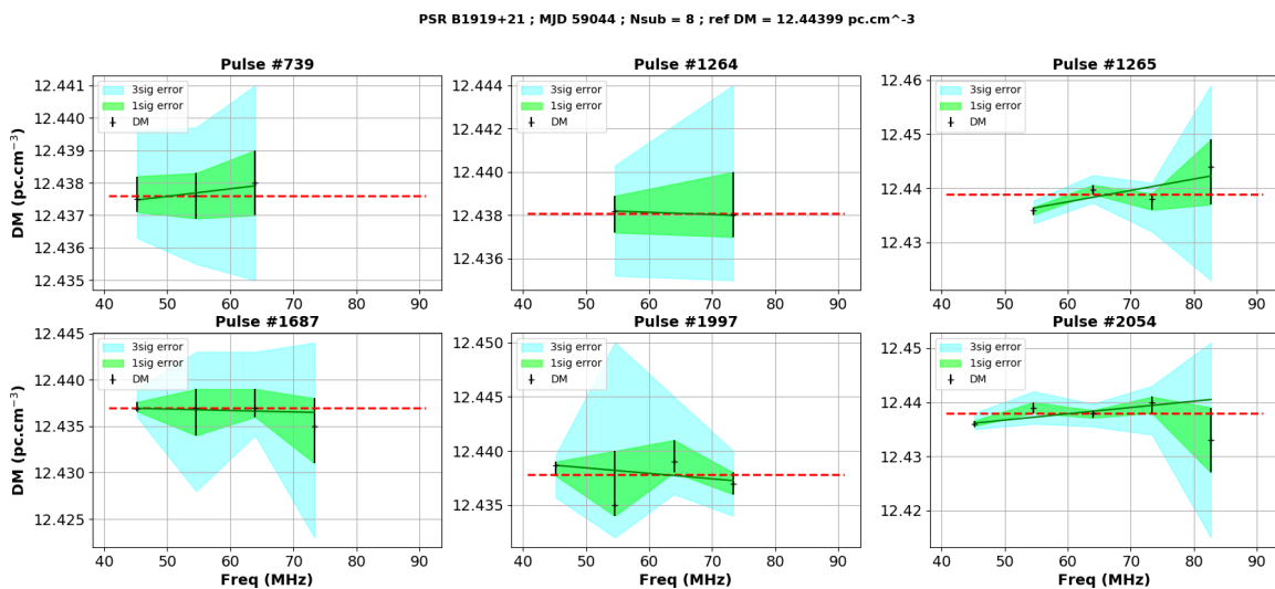
Figure 11.10: DM measurements of the different subbands for the six most intense pulses of the observation of B1919+21 at the MJD 59044.
