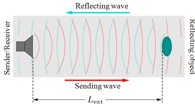
Figure 1.2: Principle of sonar distance measurement.
