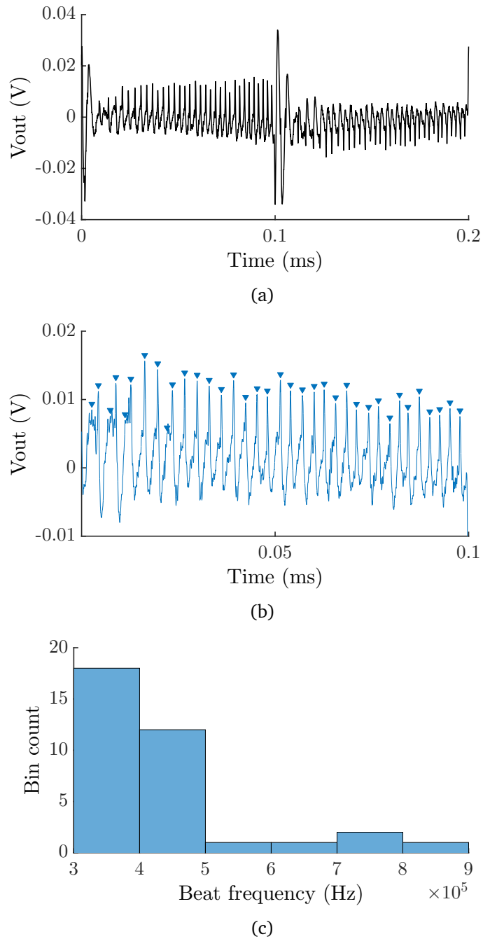
Figure 4.23: (a) Experimental results of SMI distance signal for one cycle of the triangle waveform. (b) Peaks detection of half-period of the triangular SMI waveform. (c) Histogram of beat frequencies resulting peak detections in (b).
