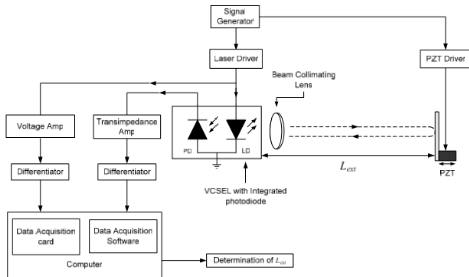
Figure 1.14: Block diagram of experimental result, signals from the photodetector and laser junction voltage are used to determine the distance between the laser and the target [6].
