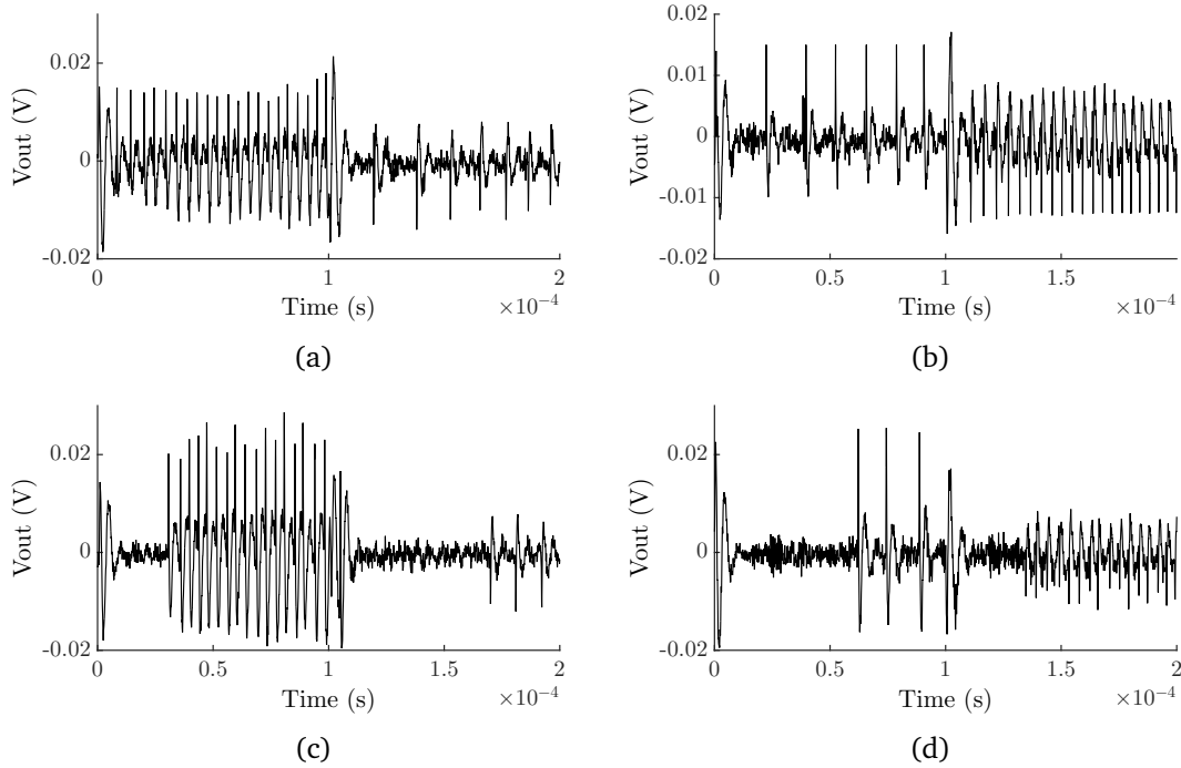
Figure 4.20: Experimental SMI signal acquisition when the distance beat frequency is superior to the Doppler frequency in different velocity directions and target surfaces. (a) and (b) The target as a white paper surface rotates in clockwise and anticlockwise, respectively. (c) and (d) The target as a micropriism reflective tape surface rotates in clockwise and anticlockwise, respectively.
