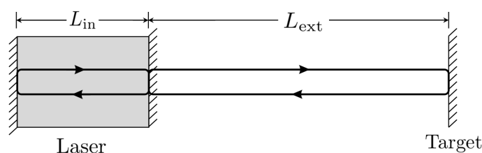
Figure 1.8: Principle of Self-Mixing interferometry.
