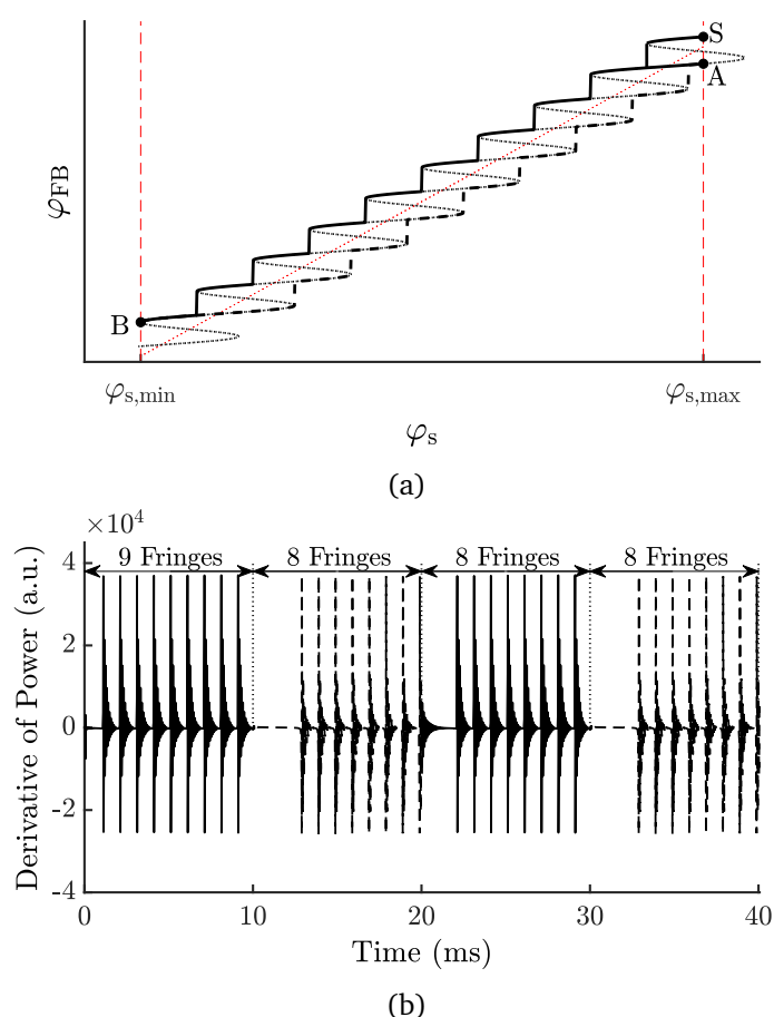
Figure 3.5: Simulation of output power from the rate equations under feedback parameter C = 6.97 . (a) Plot of the phase response \varphi_{FB} in function of the phase stimulus \varphi_s ; the thick solid and broken lines indicate the direction of the phase stimulus during decreasing and increasing respectively. (b) Plot of derivative of output power resulting from the evolution of the phase in (a).
