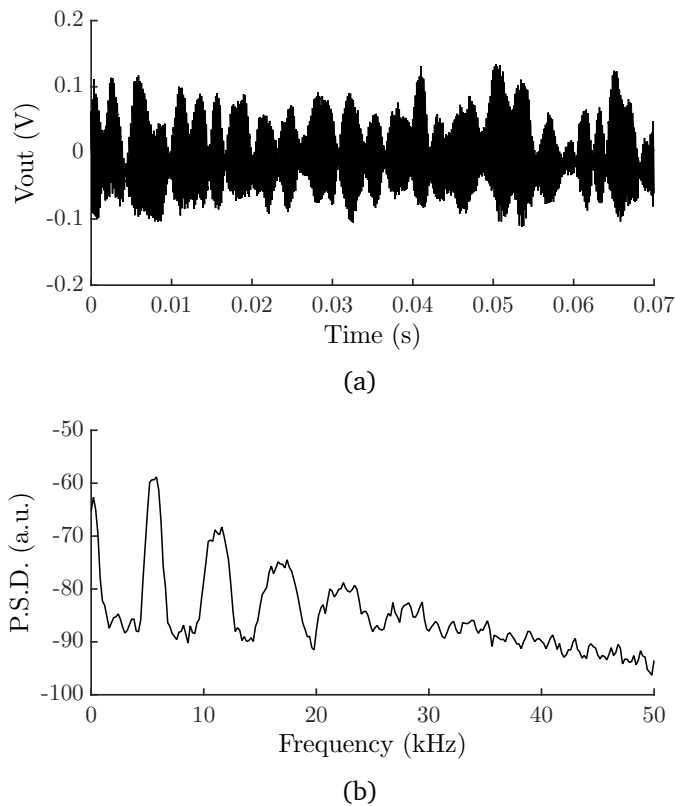
Figure 4.6: Experimental results of Doppler shift with the white paper surface. (a) The self-mixing signal in the time domain. (b) PSD of the self-mixing power variations obtained from (a).
