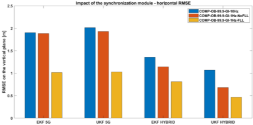
Figure 7.15 – Synchronization module impact – horizontal RMSE
