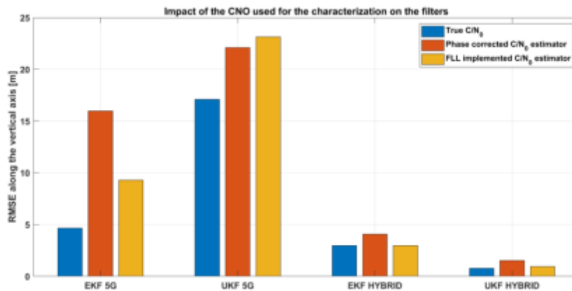
Figure 7.24 – Comparison of filters performance – C/N_0 estimator impact – RMSE along the vertical axis
