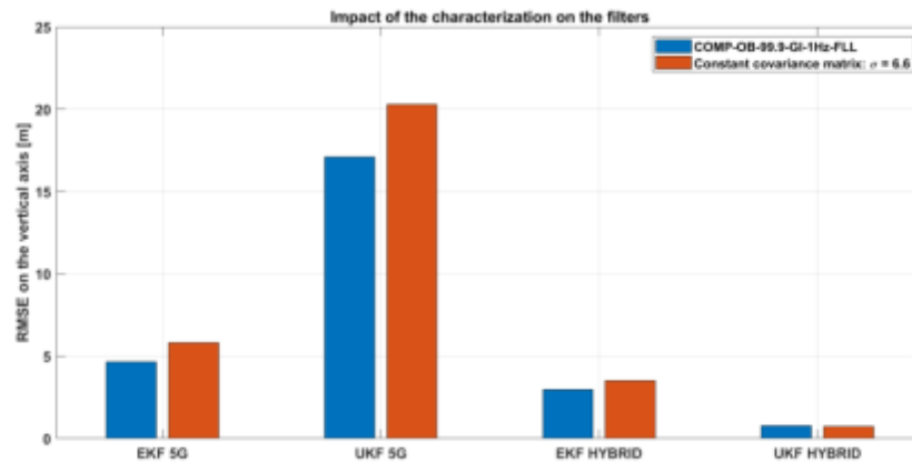
Figure 7.22 – Comparison of filters performance – characterization impact – RMSE along the vertical axis
