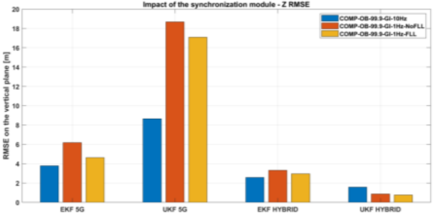
Figure 7.16 – Synchronization module impact – vertical RMSE
