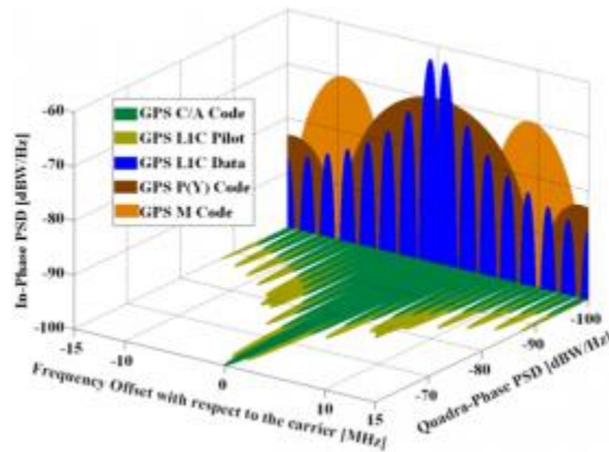
Figure 2.11 – GPS L1 signals – source [19]
