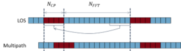
Figure 3.20 – OFDM combats time dispersity
