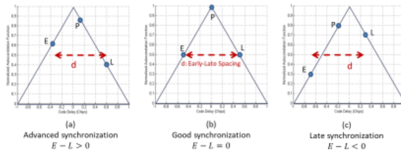
Figure 2.25 – DLL principle
