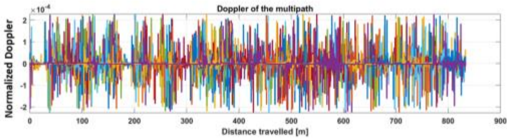
Figure 5.24 – Doppler evolution for the radial trajectory
