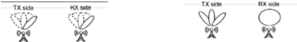
Figure 3.8 – Analogue (left) versus digital (right) beam-forming
