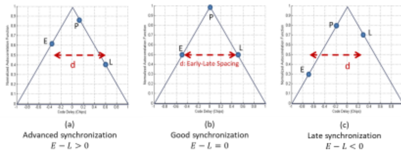
Figure 2.25 – DLL principle
