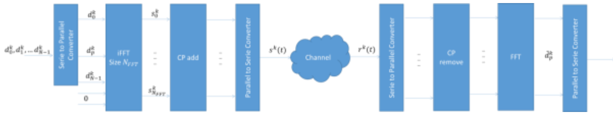
Figure 3.14 – OFDM transmission chain
