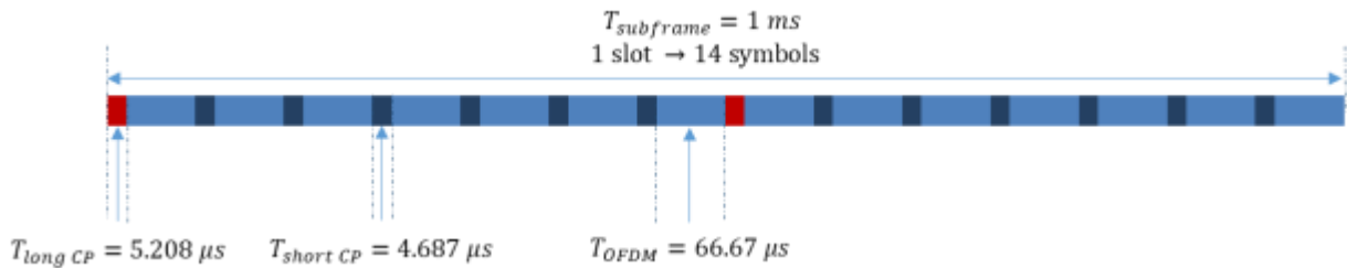
Figure 3.25 – Slot structure
