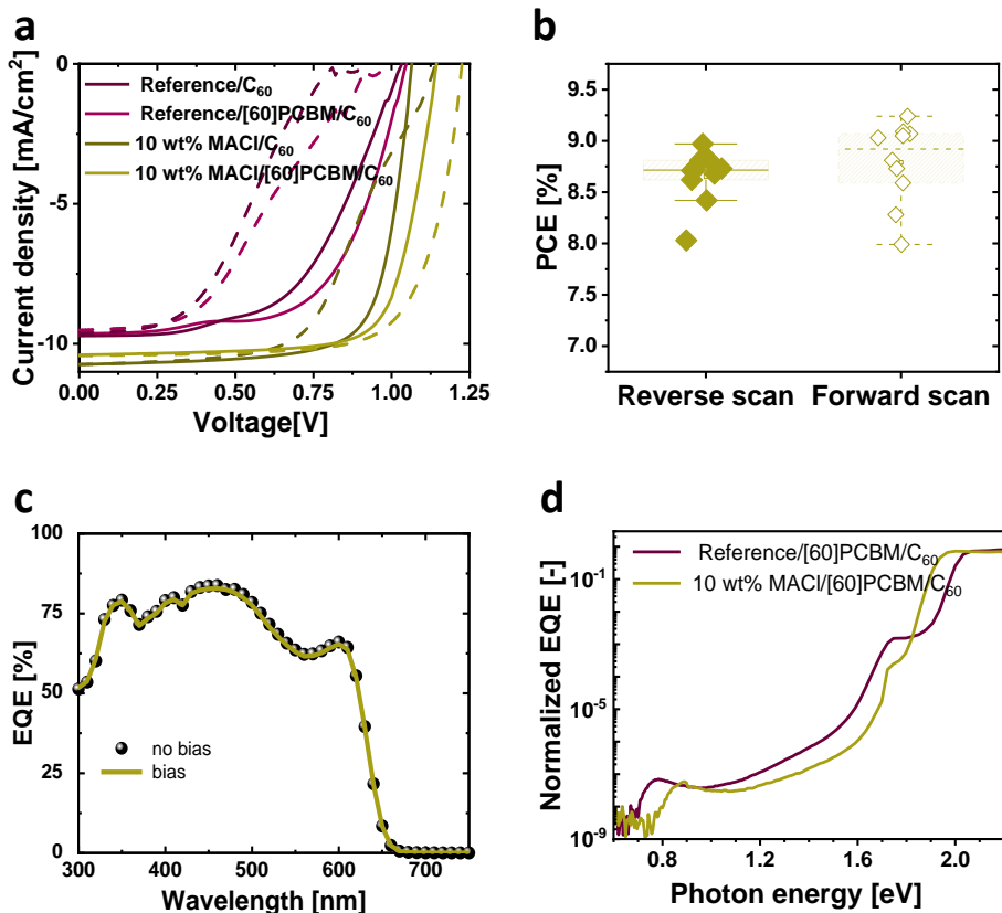
Figure 5.7. Device characterization. a) J - V characteristics for CsPbBr _{1.5} I _{1.5} and MA _{1-x} Cs _x PbI _{1.5} Br _{1.5} cells with a glass/ITO/2PACz/perovskite/ETL/BCP/Al configuration, where the ETL consists of \text{C}_{60} (40 nm) or a bilayer of PCBM (20 nm) and \text{C}_{60} (20 nm). Solid lines represent reverse scans, dashed lines forward scans. b) PCE statistics for glass/ITO/2PACz/MA _{1-x} Cs _x PbI _{1.5} Br _{1.5} /PCBM/ \text{C}_{60} /BCP/Al devices. Average PCEs are 8.7% (reverse) and 8.8% (forward). c) External quantum efficiency (EQE) spectrum of the best MA _{1-x} Cs _x PbI _{1.5} Br _{1.5} solar cell. d) Sub-bandgap EQE spectra of CsPbBr _{1.5} I _{1.5} and MA _{1-x} Cs _x PbI _{1.5} Br _{1.5} solar cells using PCBM/ \text{C}_{60} as ETL. The CsPbBr _{1.5} I _{1.5} cell shows an Urbach energy E_U = 20.8 meV, which decreases to E_U = 17.0 meV for the MA _{1-x} Cs _x PbI _{1.5} Br _{1.5} cell, implying lower energetic disorder near the band edge.
