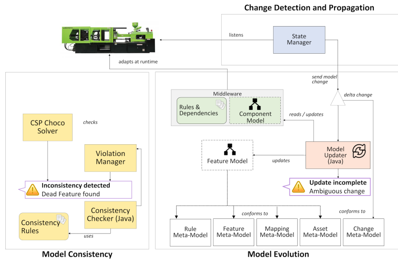
Figure 2.11: Implementation of our reference architecture for the injection molding automation system of MoldingCompany.
