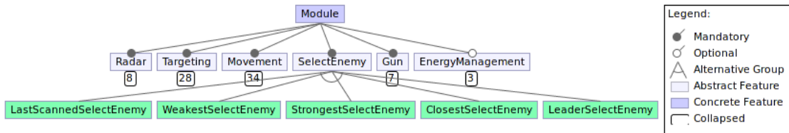
Figure 4.3: Excerpt of the Feature Model of ROBOCODESPL.
