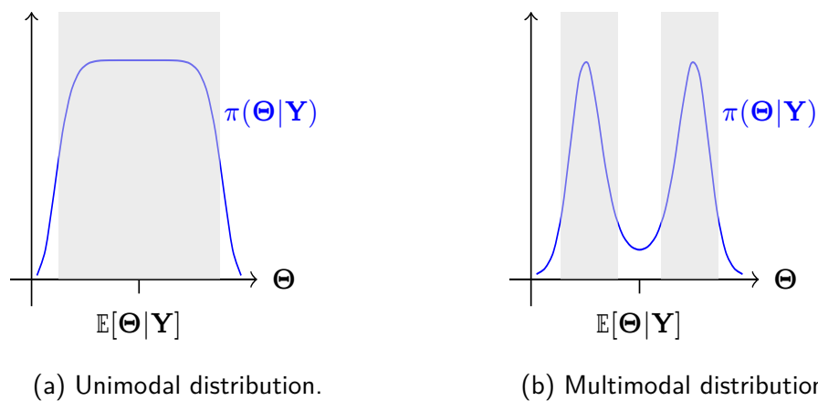
Figure 4 – Replacing a loss function by a posterior distribution. The gray areas represent high probability regions that define credibility intervals. They can be obtained with a Bayesian sampling approach.
