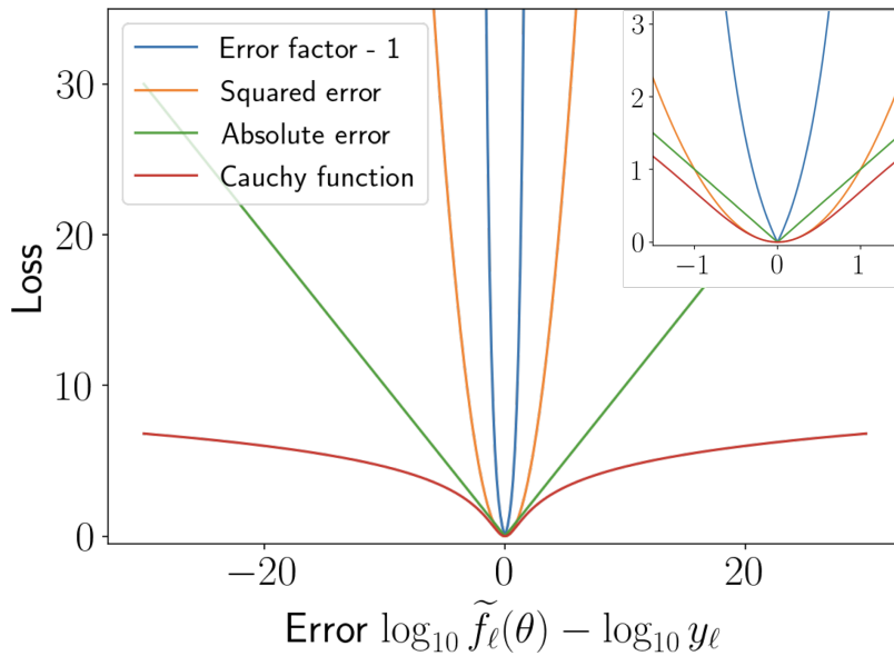
Figure 4.8 – Evolution of errors penalization by the considered loss functions. To simplify the visualization, the errors are plotted in decimal log scale, while the surrogate models train on the natural log scale. An error of 30 thus corresponds to a factor of 10^{30} . Since some line intensities range from 10^{-50} to 10^{-2} , very high error can occur early in the training phase.
