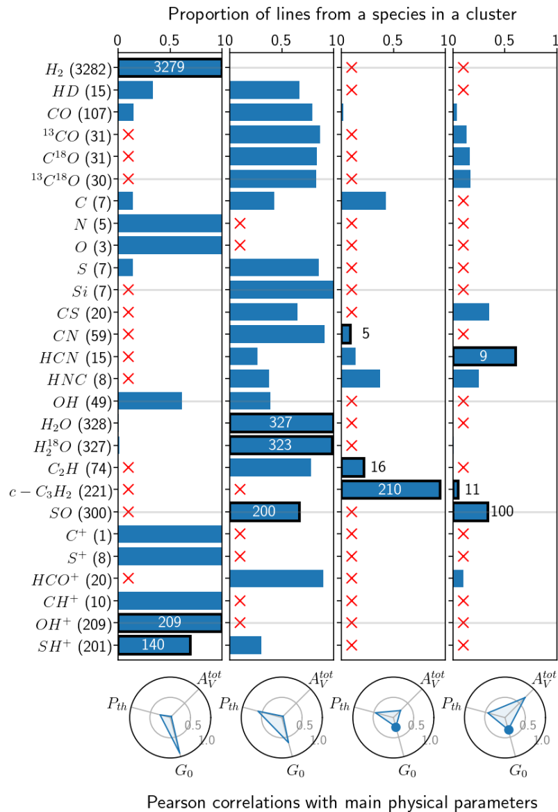
Figure 4.10 – On both top and bottom plots: each column corresponds to one of the four line clusters obtained in Section 4.6.2.
