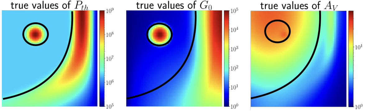
Figure 5.7 – Structure of the synthetic molecular cloud and associated true maps of physical parameters \Theta . The circle on the top left of the maps indicates a buried source. The surrounding region is a deep molecular cloud. The region on the right is a PDR illuminated by a UV source out of the image.
