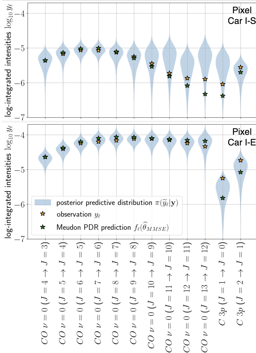
Figure 6.7 – Posterior predictive assessment two pixels of the Carina nebula on the lines used for the inversion. Comparison of observations \mathbf{Y} and associated noise model with posterior predictive distributions on \tilde{\mathbf{f}}(\Theta) , with \Theta \sim \pi(\Theta|\mathbf{Y}) . Note that these plots are imperfect as the Gaussian additive noise can lead to negative predicted observations \tilde{y}_\ell in the low SNR regime. These negative values are not displayed. For the lower intensities, underestimating the integrated intensity y_\ell may thus be compatible with the additive Gaussian noise model.
