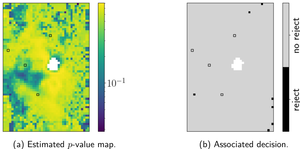
Figure 6.13 – Model assessment for OMC-1.
