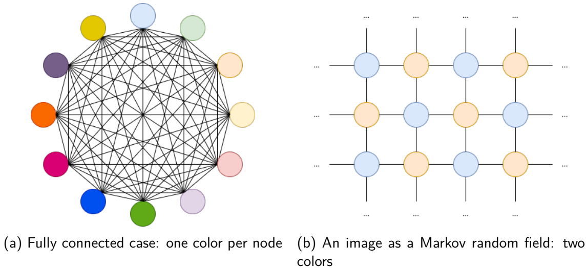
Figure 2.2 – Graphs of conditional dependence and associated optimal coloring.
