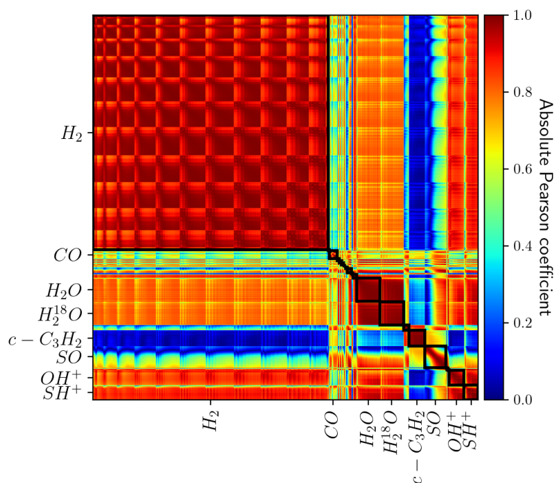
Figure 4.9 – Meudon PDR code correlations among the L = 5375 predicted lines from 27 chemical species, shown with the L \times L matrix of absolute Pearson correlation coefficients. A value of exactly 1 for two lines means that there exists an exact affine relationship between their log-intensities. The black squares on the diagonal group lines from a common chemical species. For readability reasons, only the names of species with more than 100 lines predicted by the Meudon PDR code are displayed.
