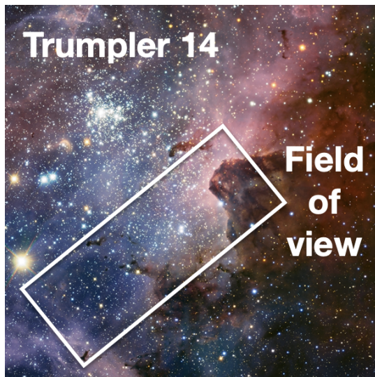
(a) Localization of the field of view with respect to the Trumpler 14 star cluster.
