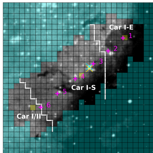
(b) Effective field of view (gray pixels). The background image is taken in the DSS2-red band. The magenta crosses indicate the pointings used during observation. The blue and yellow crosses pinpoint two massive stars. Taken from Wu et al. (2018).
