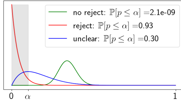
Figure 5.3 – Illustration of the three-case test for model assessment. In this case, \alpha = 0.1 and \delta = 0.1 .
