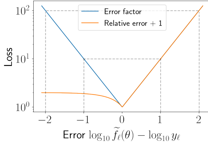
Figure 4.6 – Comparison of the error factor and the relative error. To simplify the visualization, the errors are plotted in decimal log scale, while the surrogate models train on the natural log scale. We add 1 to the relative error to simplify the comparison and to avoid a divergence of the log-relative error towards -\infty when \tilde{f}_\ell(\theta) \rightarrow y_\ell . The relative error + 1 tends to 2 for large negative errors, i.e., the relative error tends to and is upper bounded by 100%. This effect favors underestimations compared to overestimations. Using the error factor cancels this undesirable effect.
