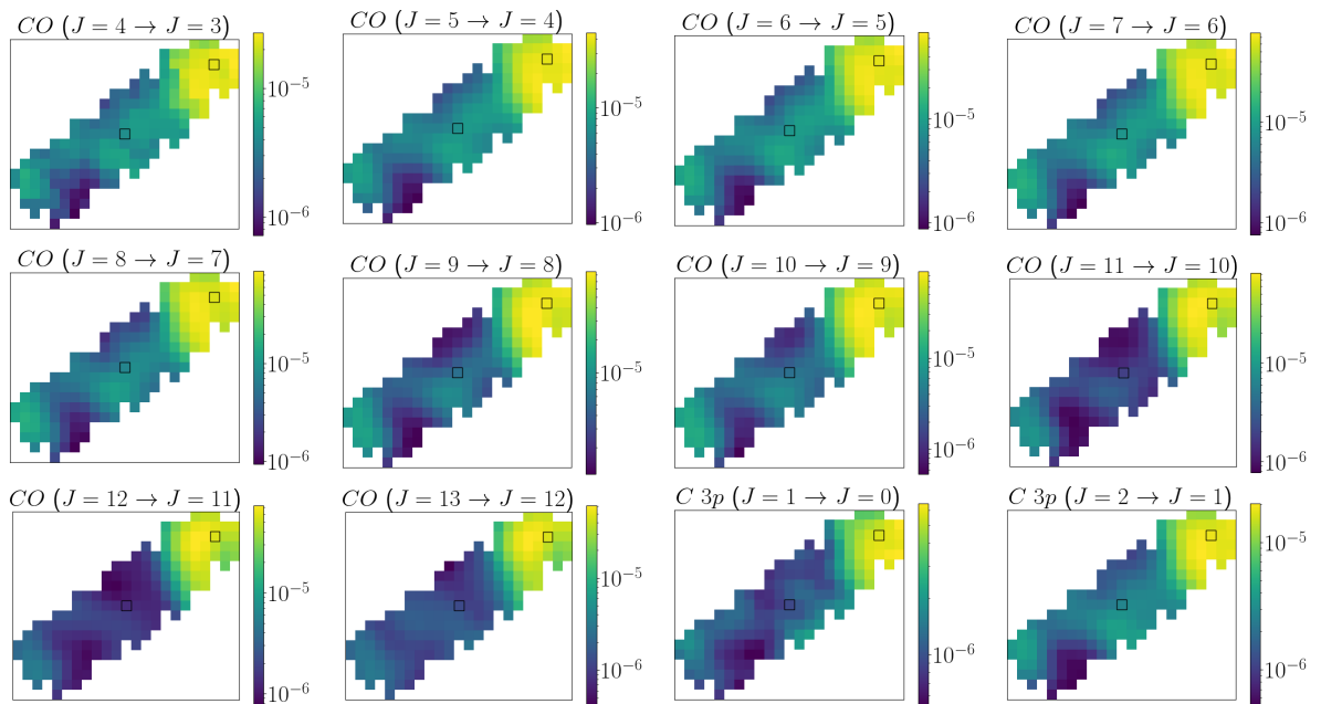
Figure 6.5 – Observations of the Carina nebula. The Car I-E is brightest for all lines, as it is directly illuminated by the Trumpler 14 star cluster.
